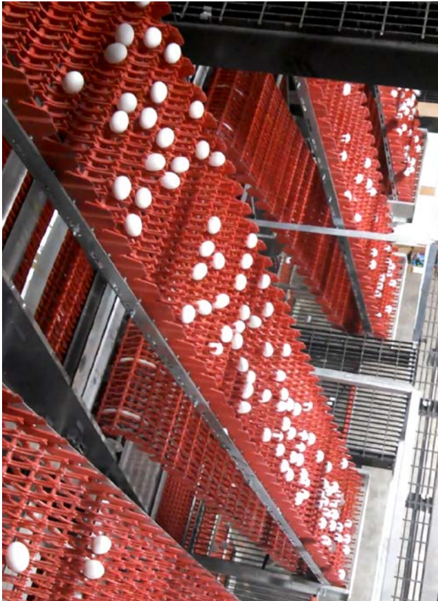
Chore-Time's EXCELSIOR® High-Capacity Collector can collect eggs from up to 16 tiers at once.
