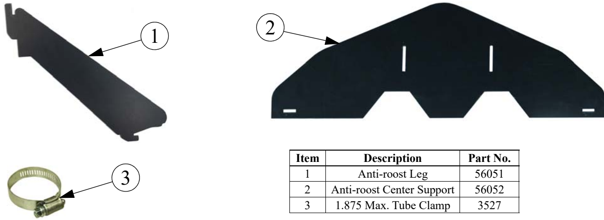
Figure 1. Part Numbers
