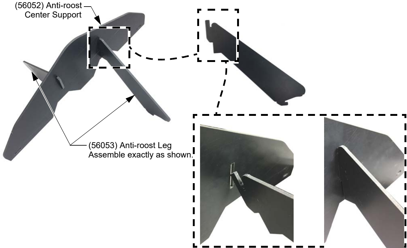
Figure 2. Assembling Anti-roost
