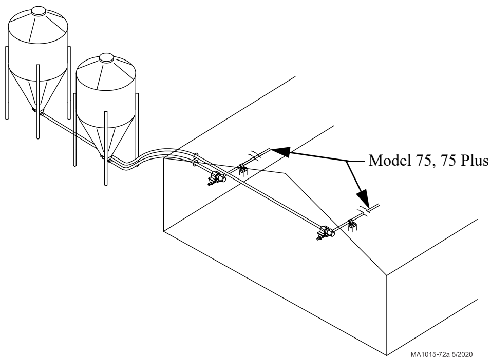
Figure 11.High Capacity Flag System Layout #2
