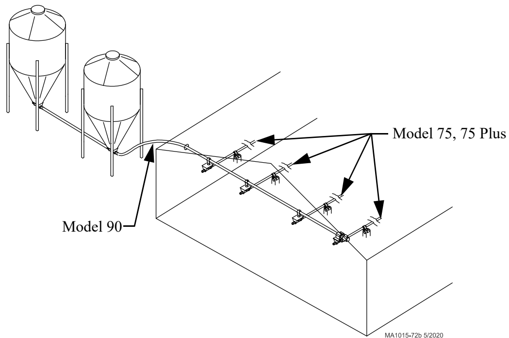
Figure 12.High Capacity Flag System Layout #3
