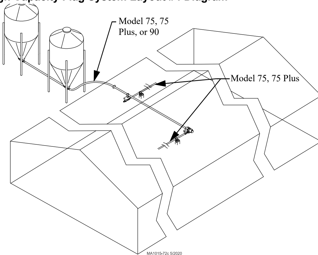
Figure 13.High Capacity Flag System Layout #4
