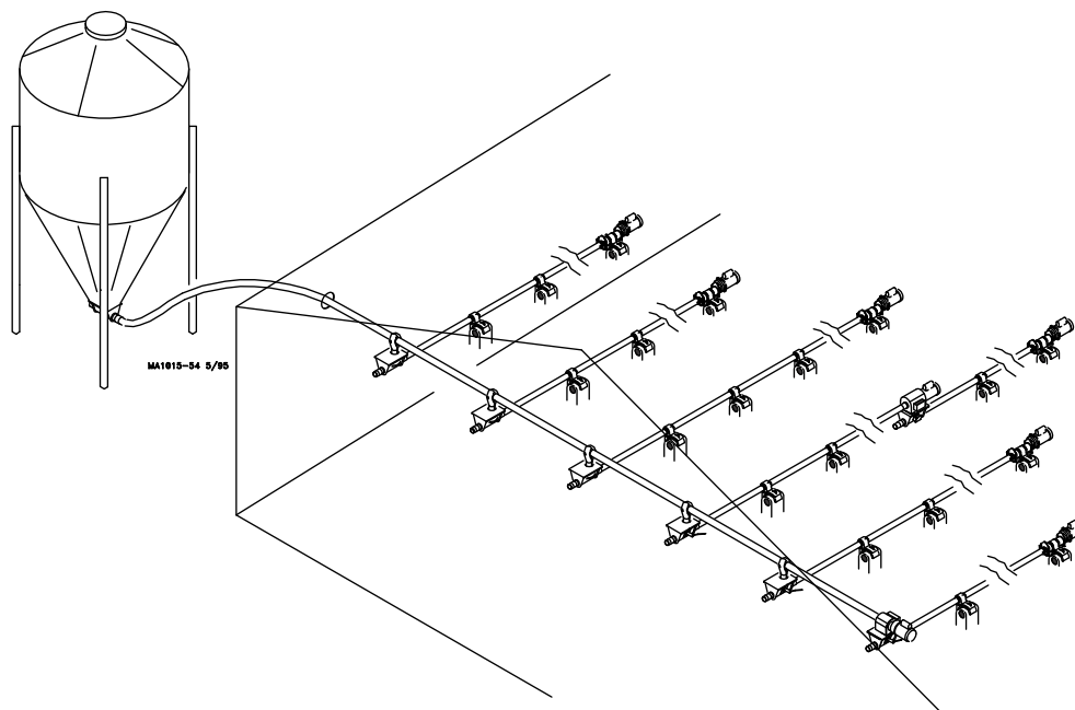
Figure 6. Standard Flag System Layout
