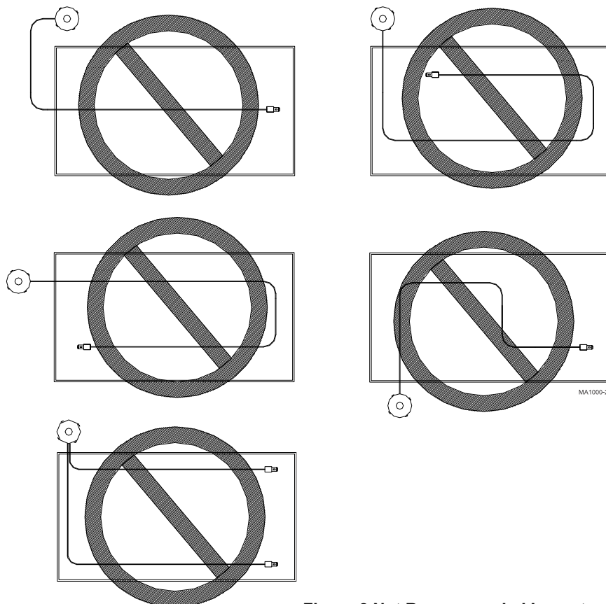
Figure 2.Not Recommended Layouts
