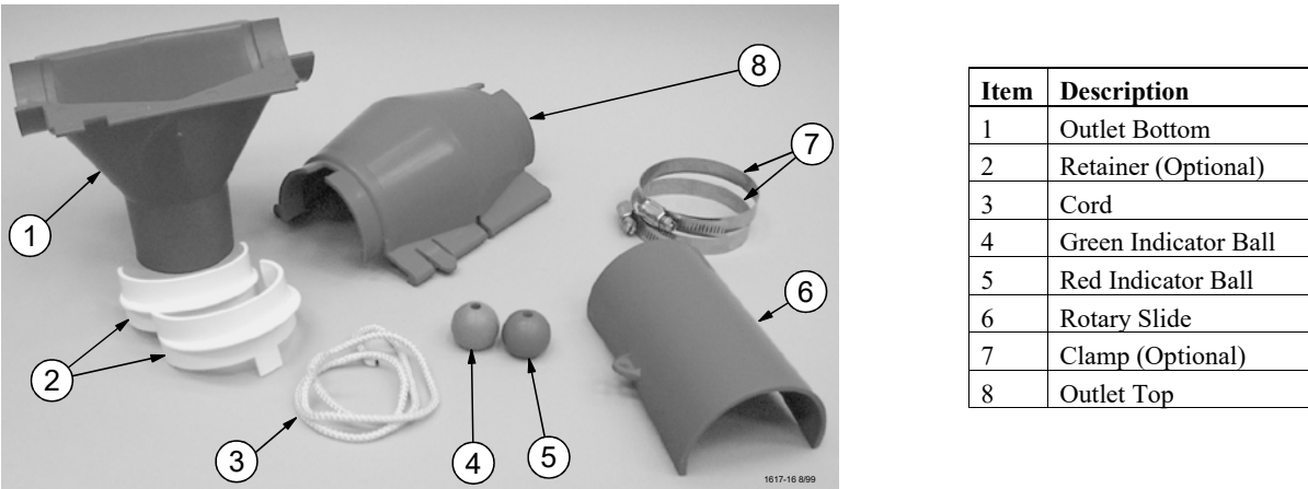
Figure 12.Outlet Assembly Components
