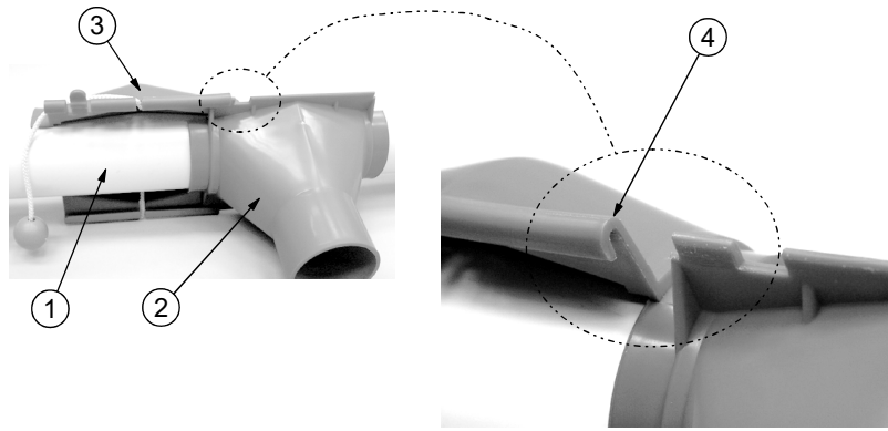
Figure 17. Assembling the Outlet Bottom to the Outlet Top
