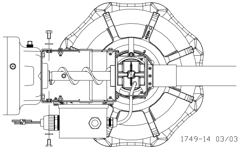
Figure 42. Attaching the Anchor Plate and Gearhead Assembly to the Control Unit Body
