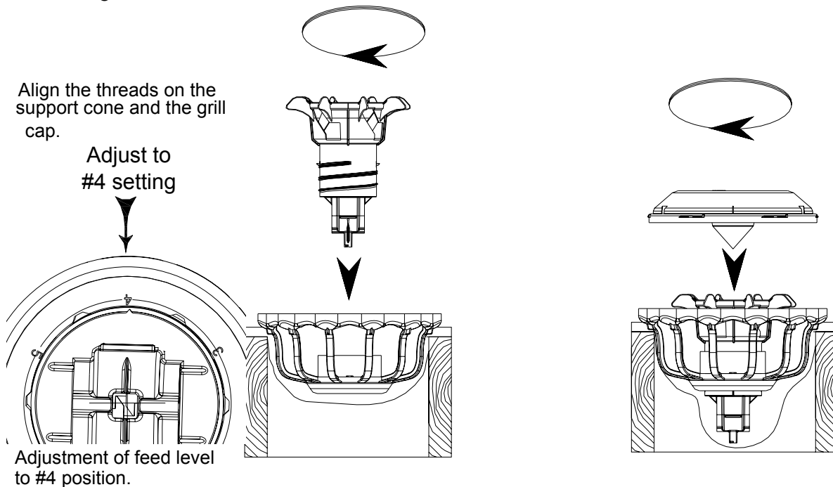
Figure 24. Pan Assembly Option 1
