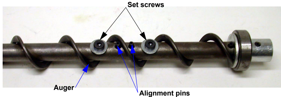
Figure 46. Auger and Anchor Bearing Connection
