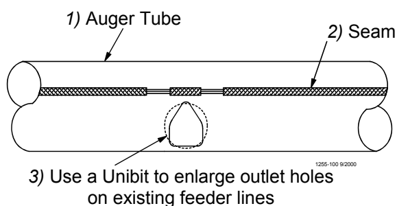
Figure 65. Enlarging Outlet Holes
