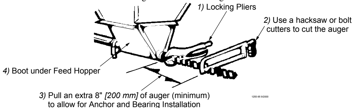
Figure 45. Cut the Auger with required stretch
