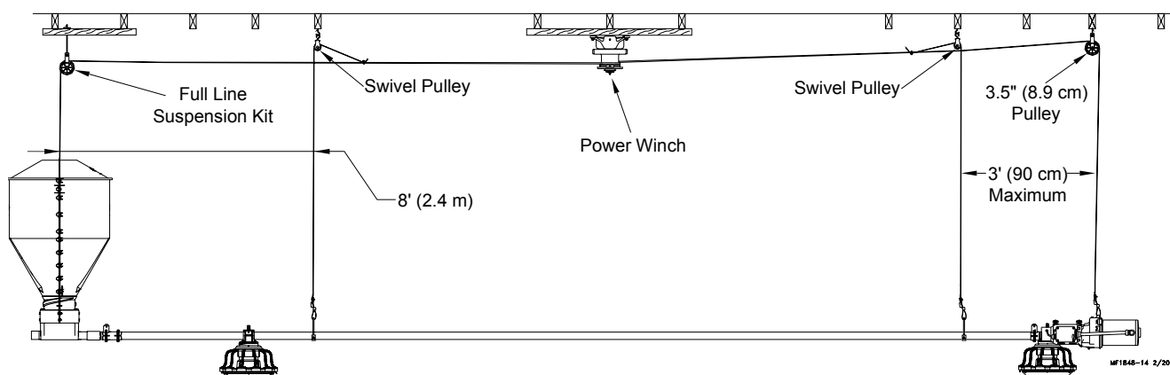
Figure 4. Suspension for systems over 350' [107 m]
