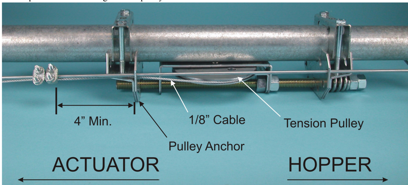
Figure 56. Cable Installation
