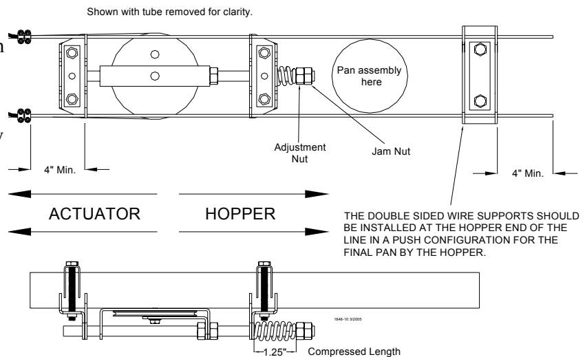
Figure 55. Pulley Assembly
