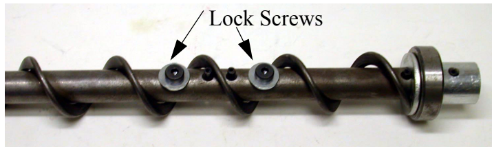
Figure 78. Auger and anchor Bearing Connection
