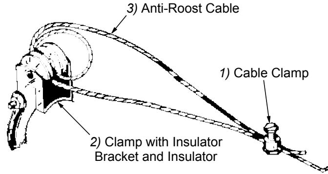
Figure 68. Anti-Roost Cable at the Hopper
