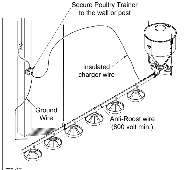
Figure 71. Poultry Trainer Installation
