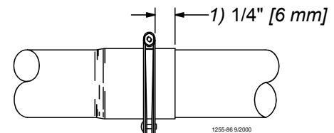
Figure 35. Clamp Installation
