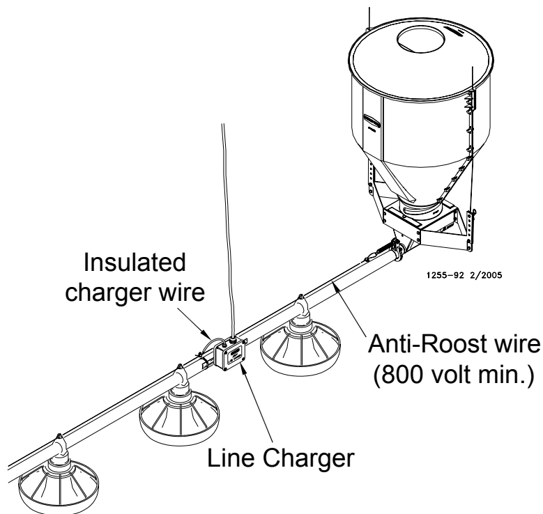
Figure 72. Line Charger Installation
