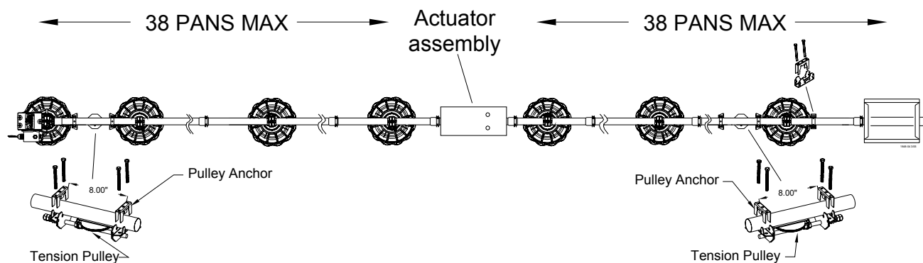
Figure 49. Tension Pulley Installation
