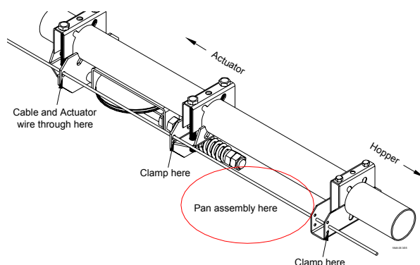
Figure 53. Installing actuator wire
