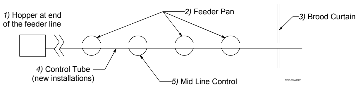
Figure 64. Figure 68 Mid-Line Control Location Diagram
