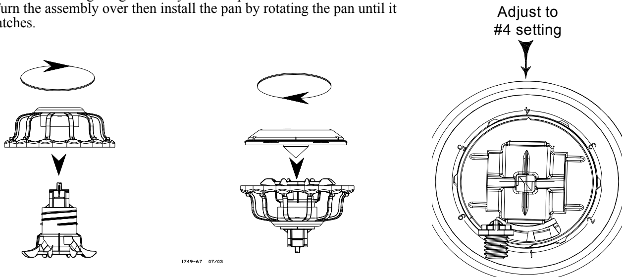
Figure 25. Pan assembly option 2
