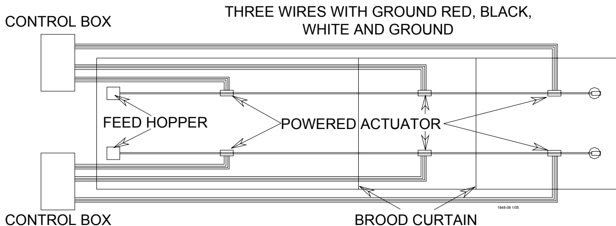
Figure 57. Powered Actuator House Wiring layout
