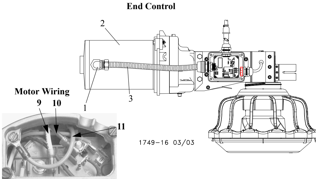
Figure 43. Wiring the Motor
