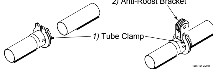
Figure 34. Tube Clamp and Tube Clamp with Anti-Roost Bracket
