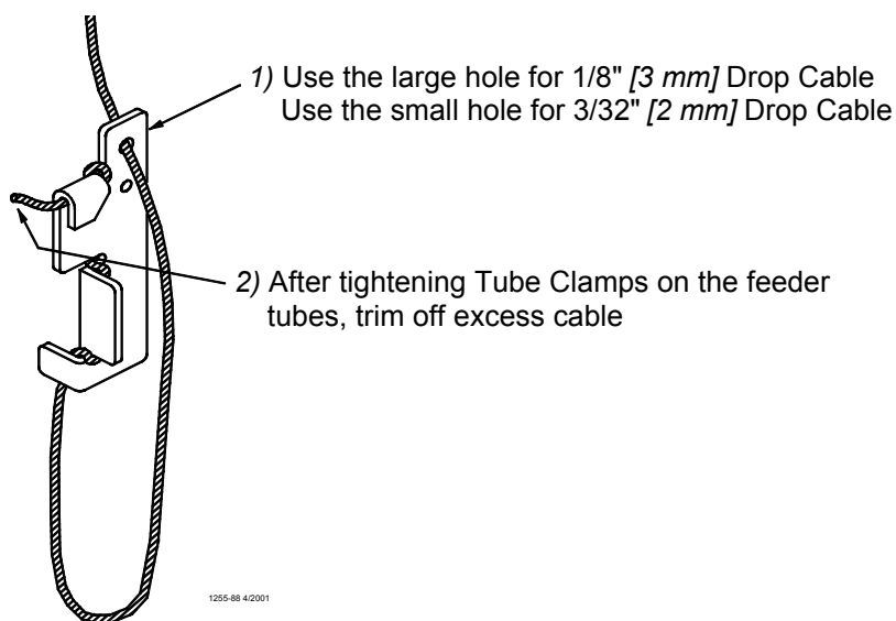
Figure 37. Cable Lock Threading
