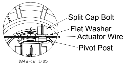
Figure 59. 13057 clamp installed
