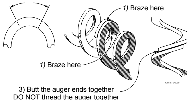
Figure 47. Auger Brazing
