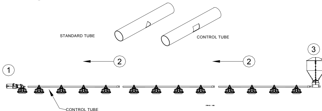
Figure 32. Attaching Feeder Tube Assemblies
