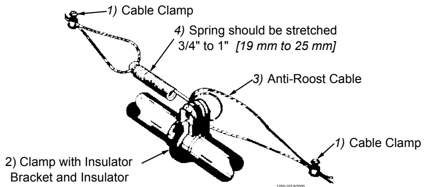
Figure 68. Anti-Roost Cable at the Hopper
