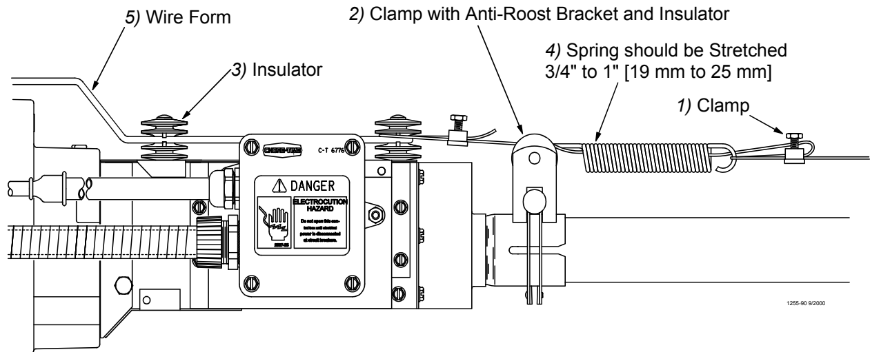
Figure 70. Anti-Roost Installation at the Control Unit
