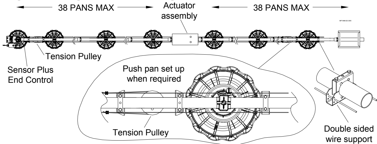
Figure 29. Feeder layout
