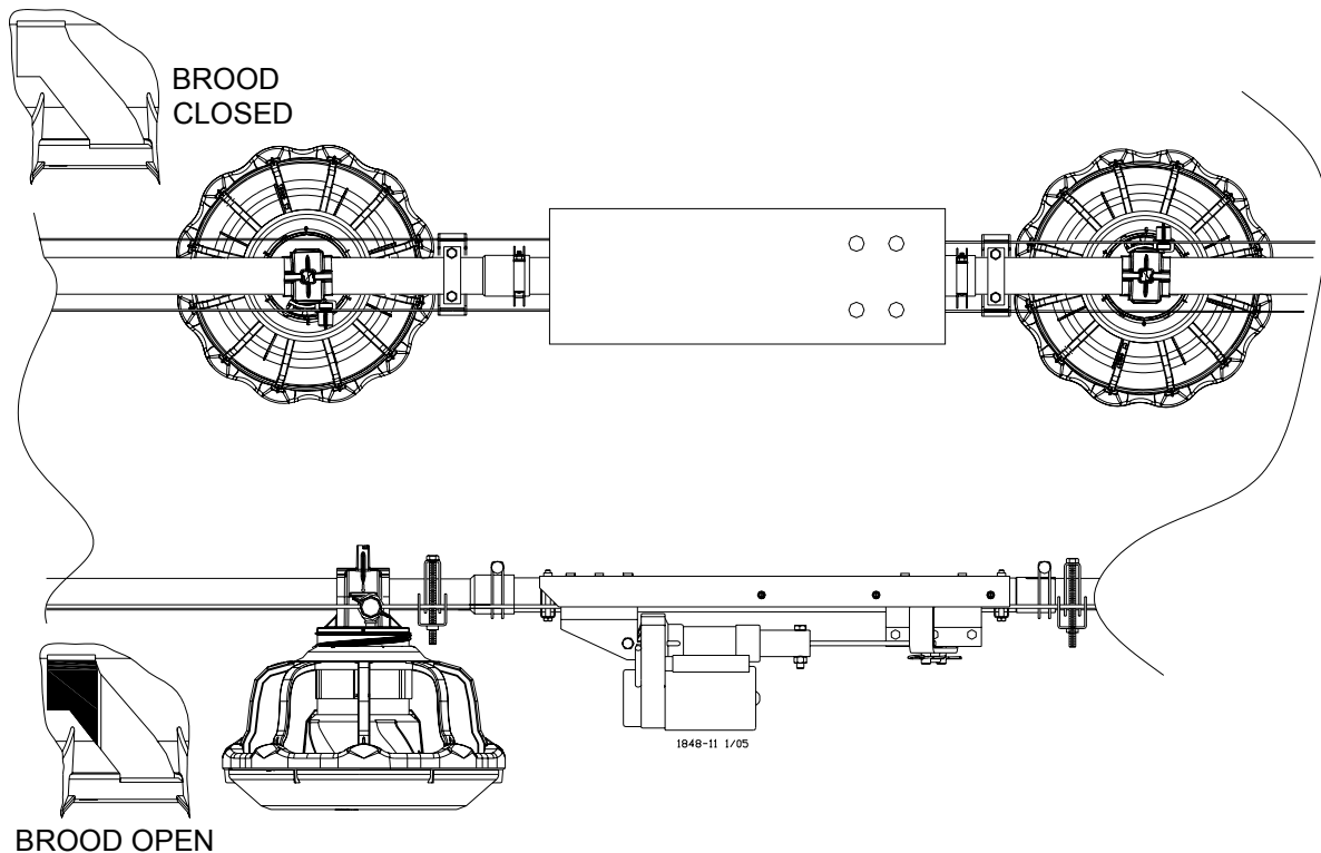
Figure 62. Adjusting the Vari-Brood opening
