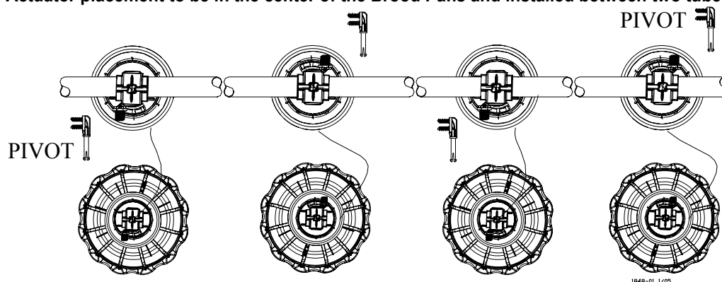
Figure 28. Pan orientation on feeder tube.
