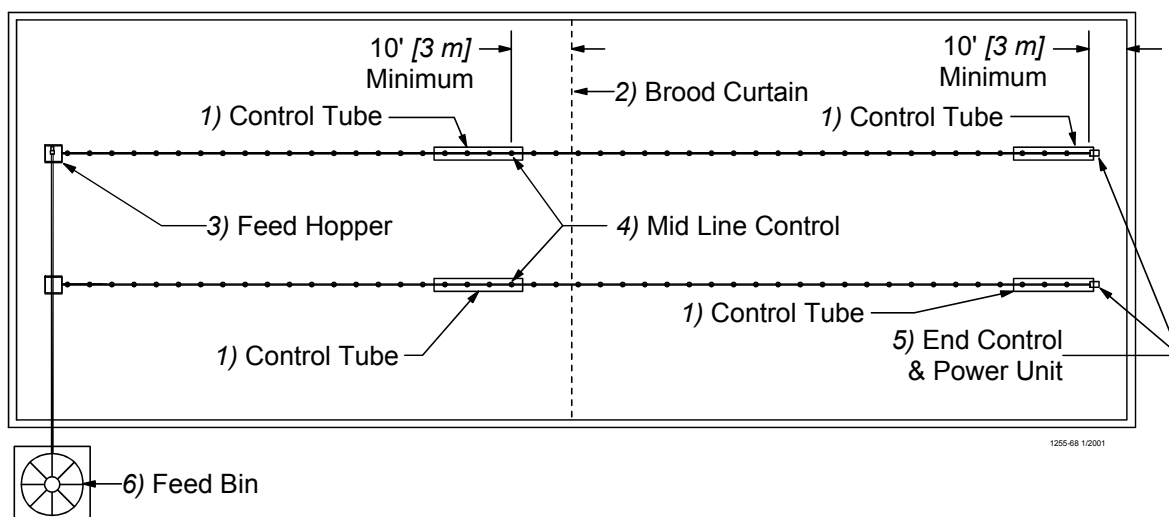
Figure 74. Component location diagram for systems up to 400 feet [122 m]. (Top View).
