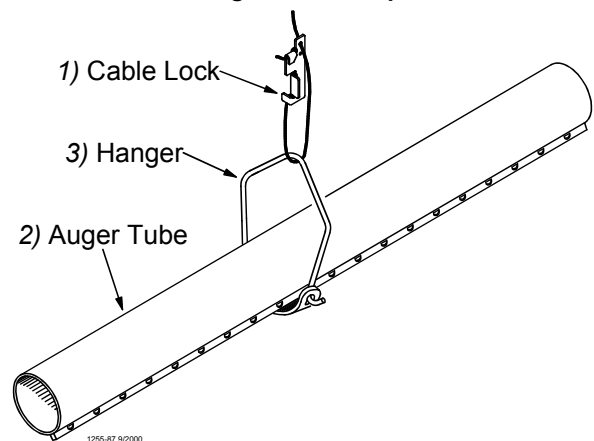
Figure 36. Hanger Installation
