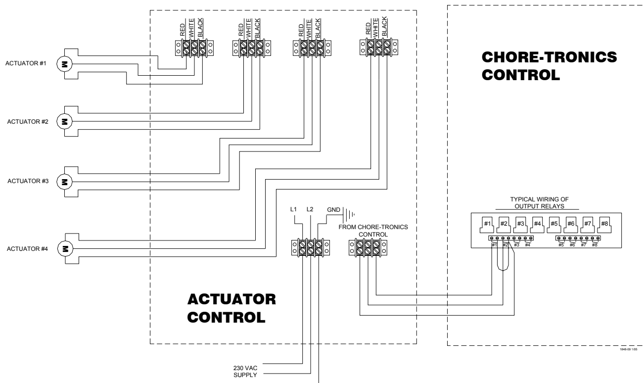
Figure 58. Powered Actuator Wiring
