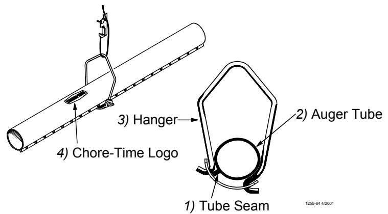
Figure 33. Hanger Installation
