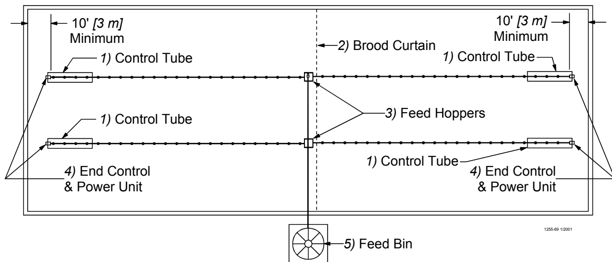
Figure 73. Component location diagram for systems over 400 feet [122 m]. (Top View).
