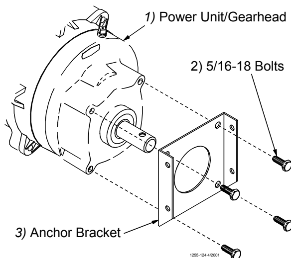
Figure 40. Assemble the Anchor Bracket to the Power Unit/Gearhead
