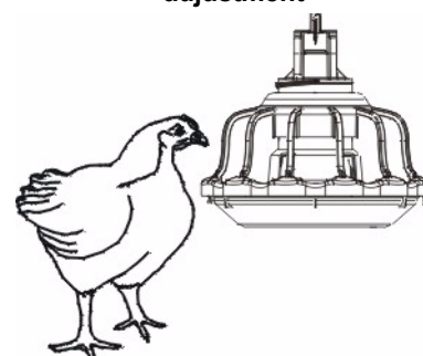
Figure 82. Feeder Pan Assembly height adjustment
