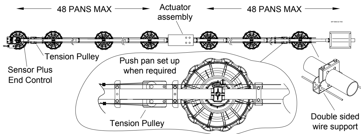
Figure 30. Feeder layout
