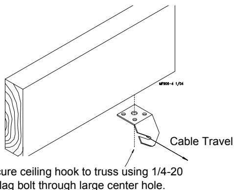
Figure 17. Wood Truss Ceiling Bracket Installation
