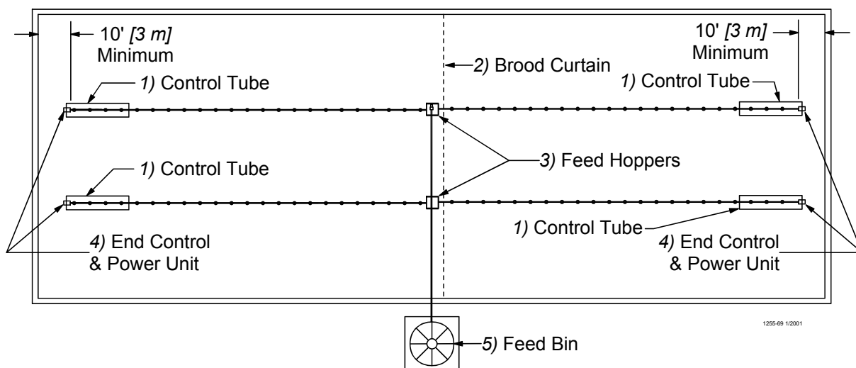
Figure 79. Component location diagram for systems over 400 feet [122 m]. (Top View).
