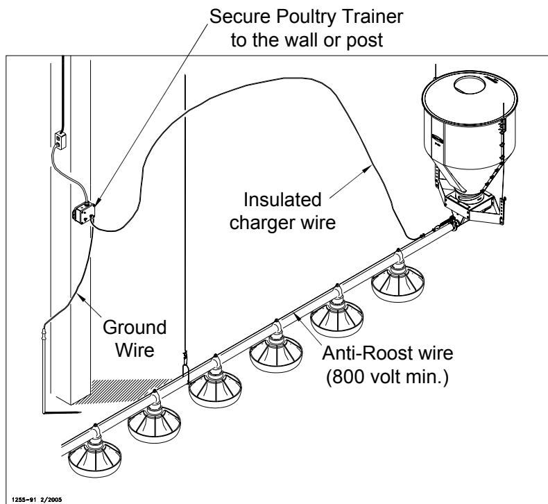
Figure 77. Poultry Trainer Installation
