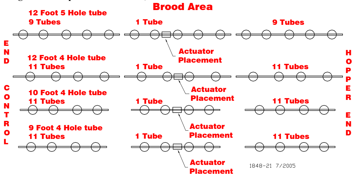
Figure 28. Typical building layout for Actuator placement.
