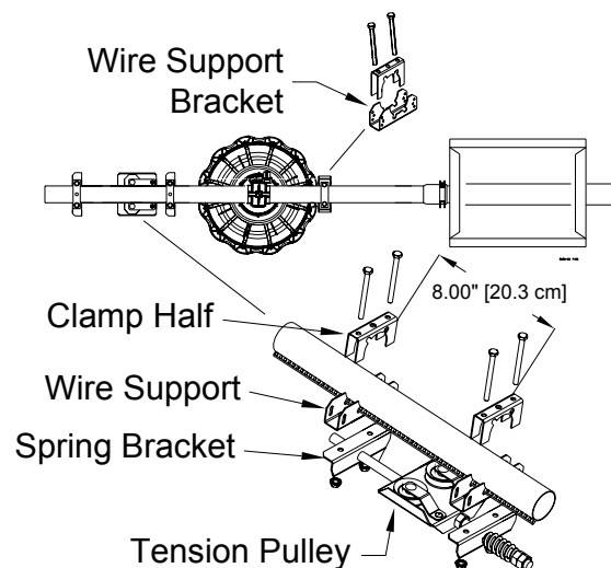
Figure 50. Tension Pulley
