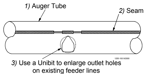
Figure 71. Enlarging Outlet Holes
