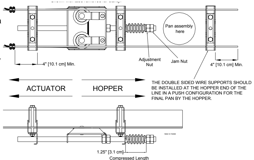
Figure 58. Pulley Assembly
