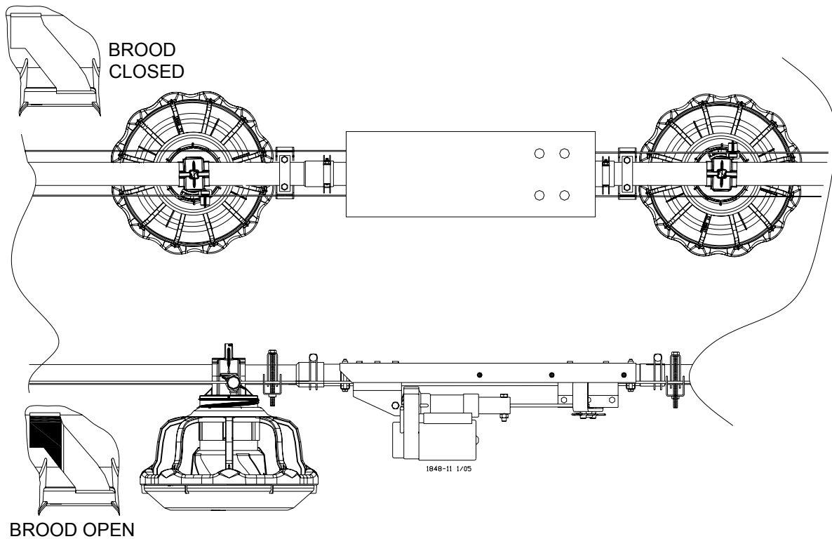
Figure 66. Adjusting the Vari-Brood opening
