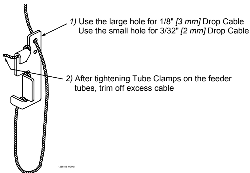
Figure 39. Cable Lock Threading
