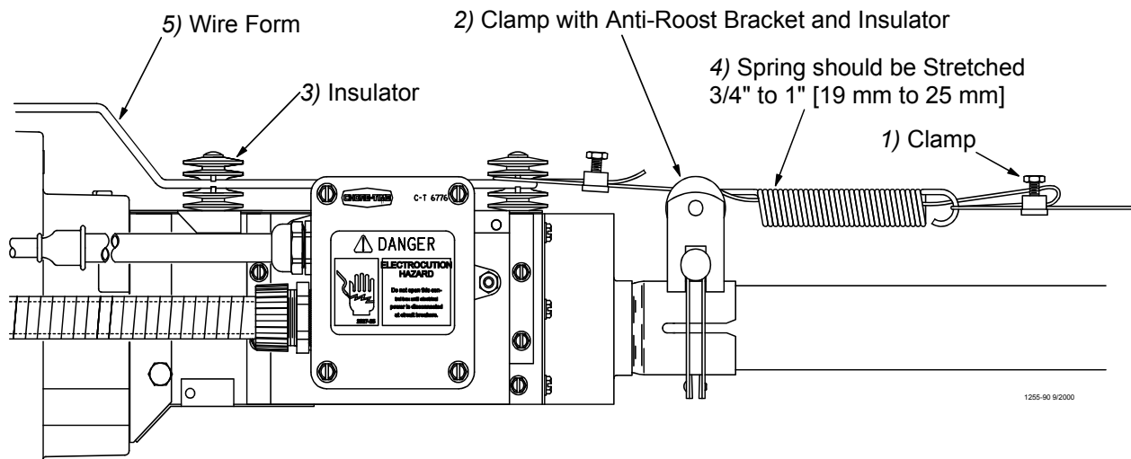
Figure 76. Anti-Roost Installation at the Control Unit
