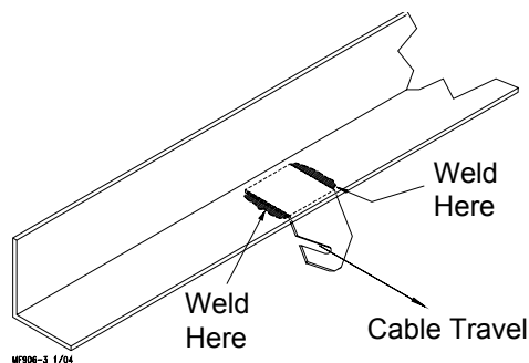
Figure 16. Welded Steel Truss Ceiling Bracket Installation
