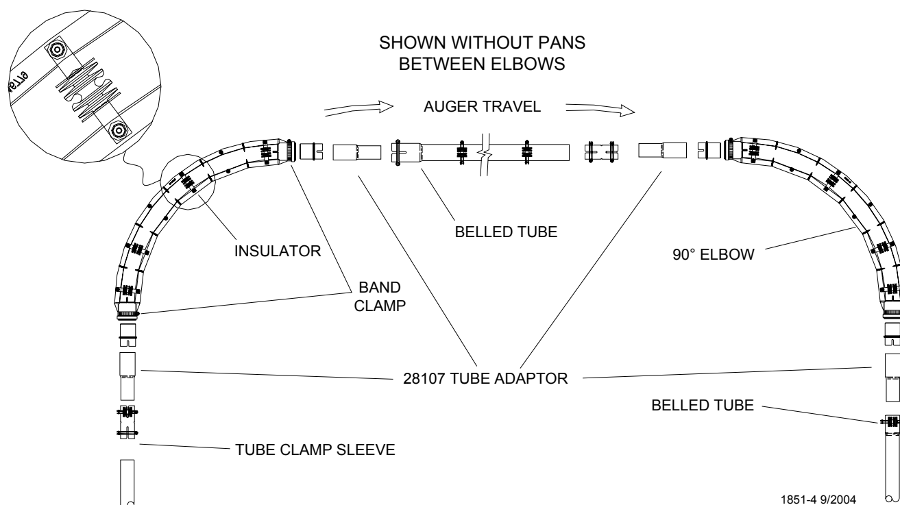
Figure 30. Install Insulators approximately as shown.
