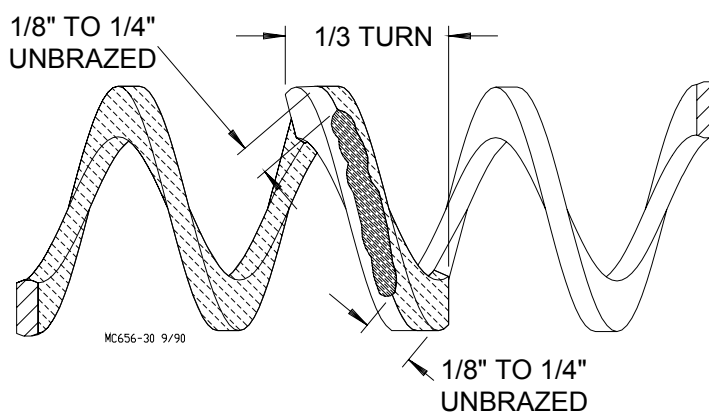
Figure 36. Brazing Area
