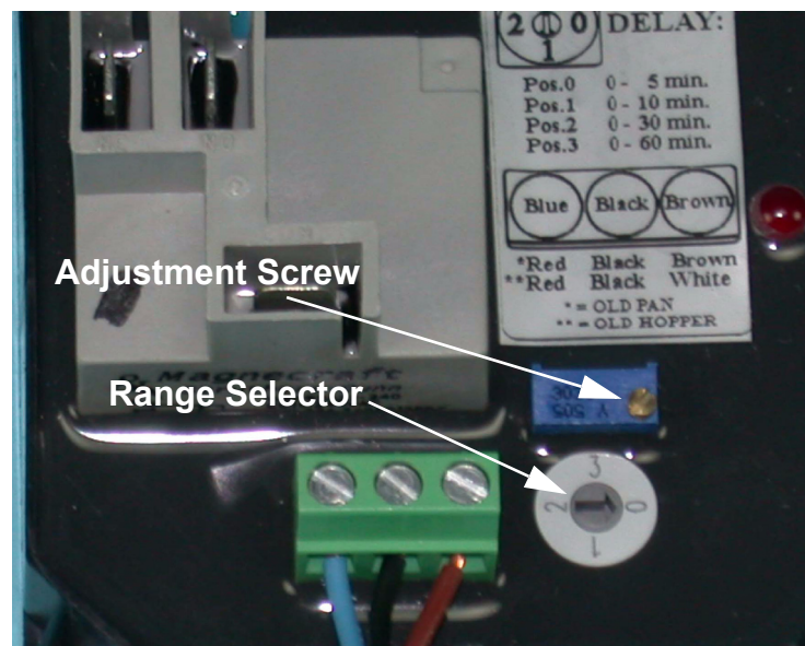
Figure 55. Adjusting the Sensor Plus Proximity Switch
