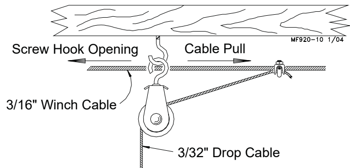
Figure 4. Screw Hook Installation
