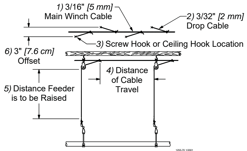
Figure 3. Drop line offset detail
