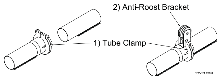
Figure 51. Tube Clamp and Clamp/Anti-Roost Bracket
