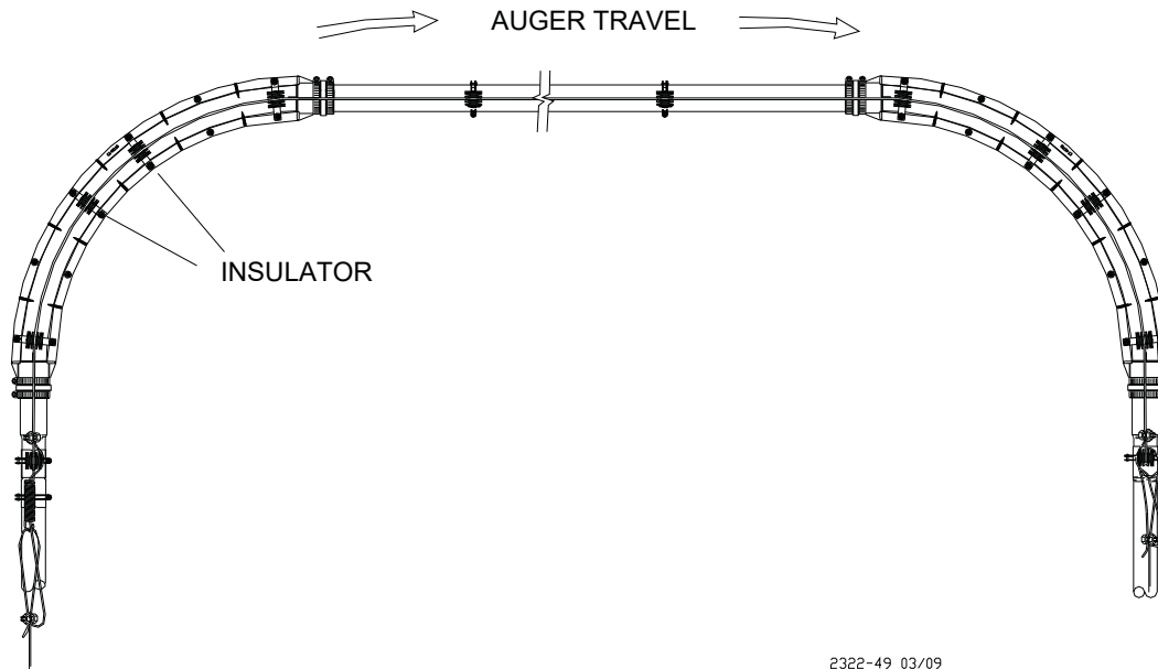
Figure 57. Anti-Roost Installation at Elbows
