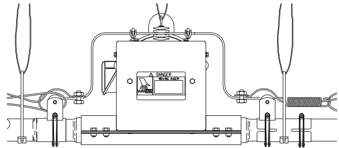
Figure 56. Anti-Roost Installation at the Drive Unit
