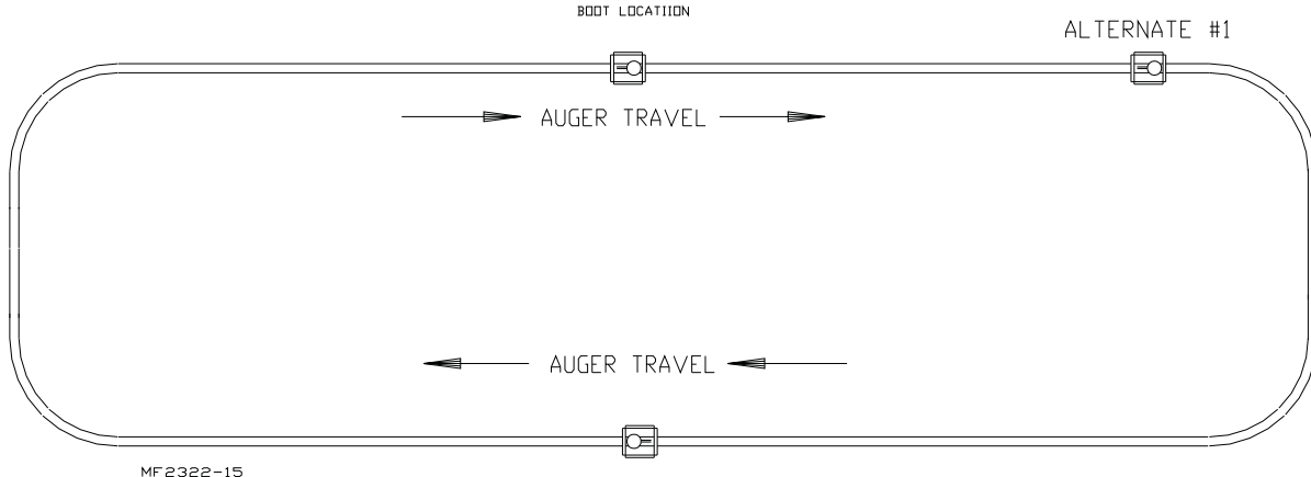
Figure 43. Feeder boot Layout
