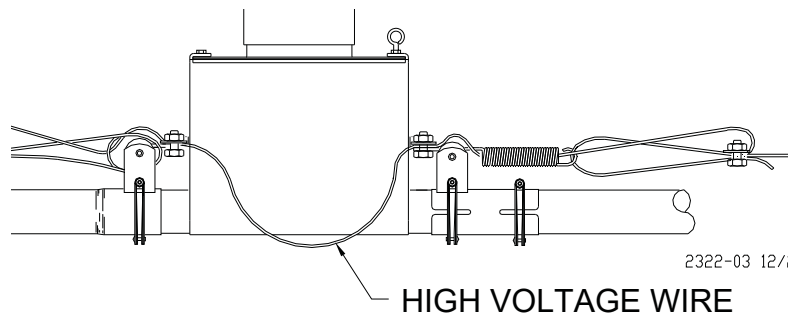
Figure 58. High Voltage Wire Installation
