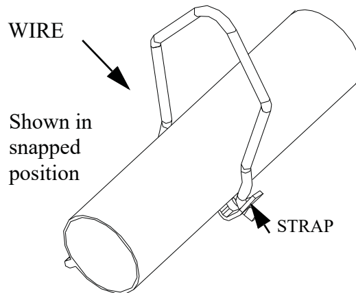
Figure 49. Hanger Installation
