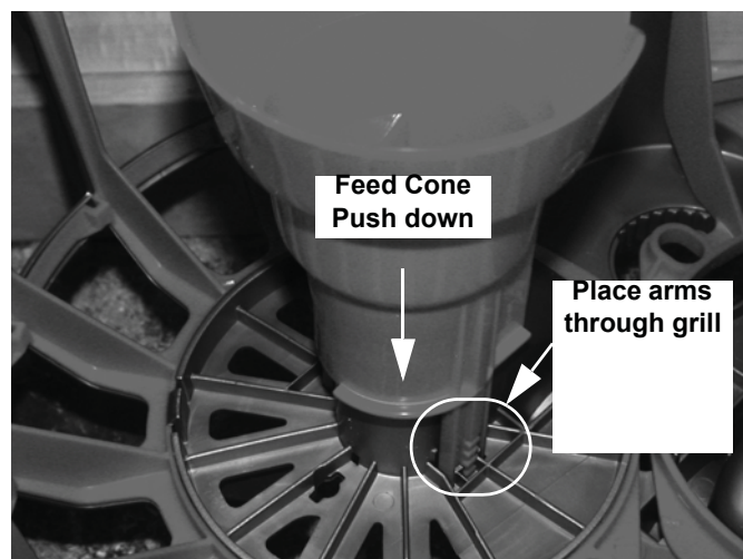
Figure 22. Install feed cones
