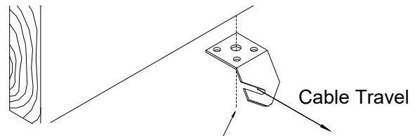
Figure 7. Welded Steel Truss Ceiling Bracket Installation
