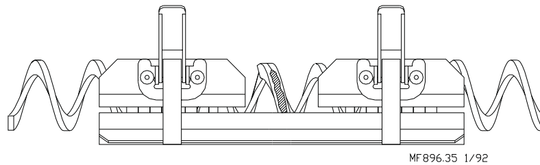
Figure 63. Welding fixture
