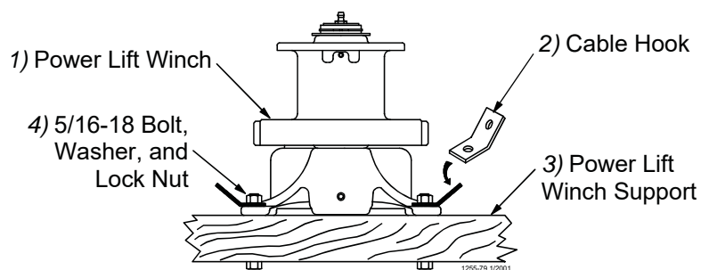
Figure 11. Assemble the Power Winch to the winch support
