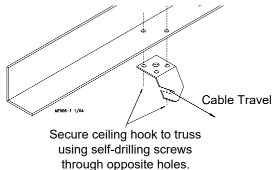
Figure 6. Steel Truss Ceiling Bracket Installation
