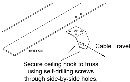
Figure 5. Narrow Steel Truss Ceiling Bracket Installation
