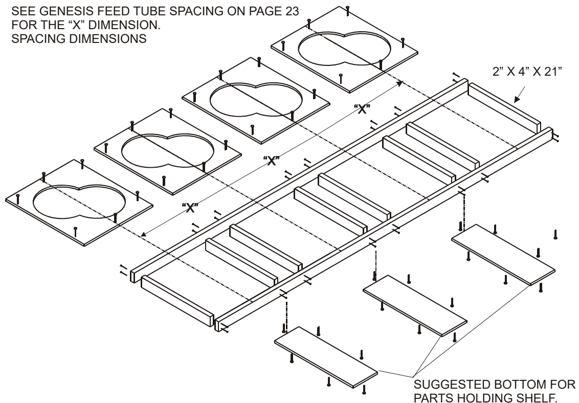
Figure 24. Feeder Pan and Tube Assembly Fixture Construction
