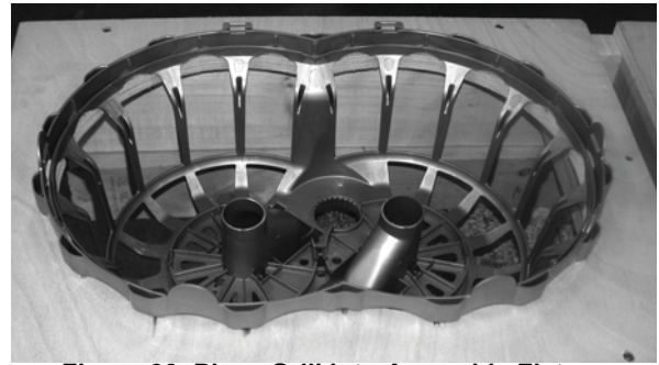
Figure 33. Place Grill into Assembly Fixture
