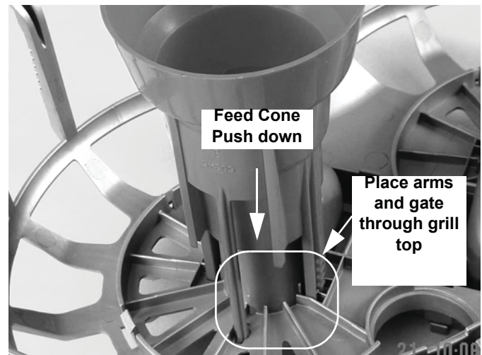
Figure 34. Install feed cones
