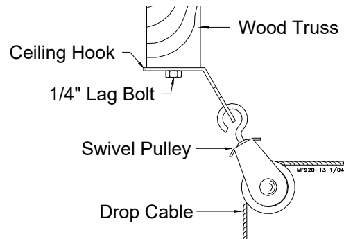
Figure 9. Pulley Installation
