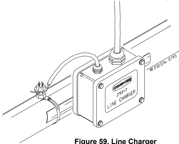
Figure 59. Line Charger Installation
