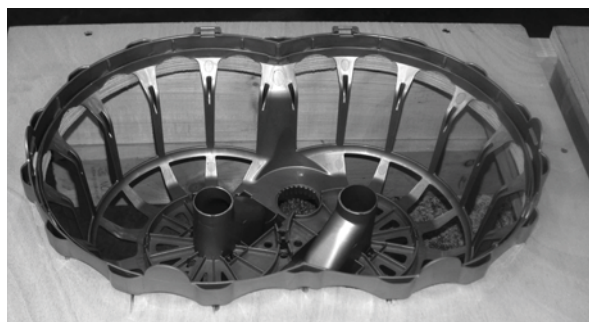
Figure 20. Place Grill into Assembly Fixture
