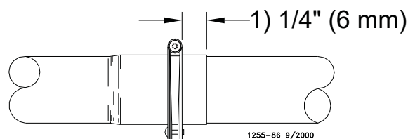
Figure 52. Tube Clamp Installation
