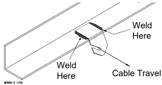
Figure 7. Welded Steel Truss Ceiling Bracket Installation
