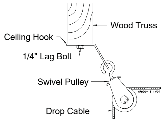
Figure 16. Feeder boot suspension.
