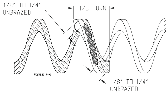
Figure 64. Brazing
