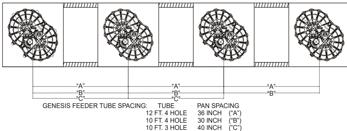
Figure 37. Pan Spacing
