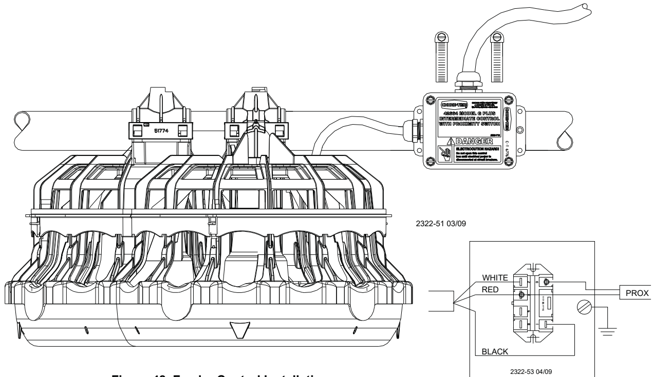
Figure 48. Feeder Control Installation
