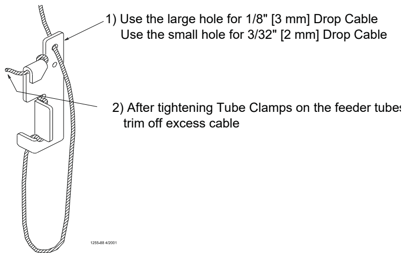
Figure 50. Adjustment Leveler Cable Threading
