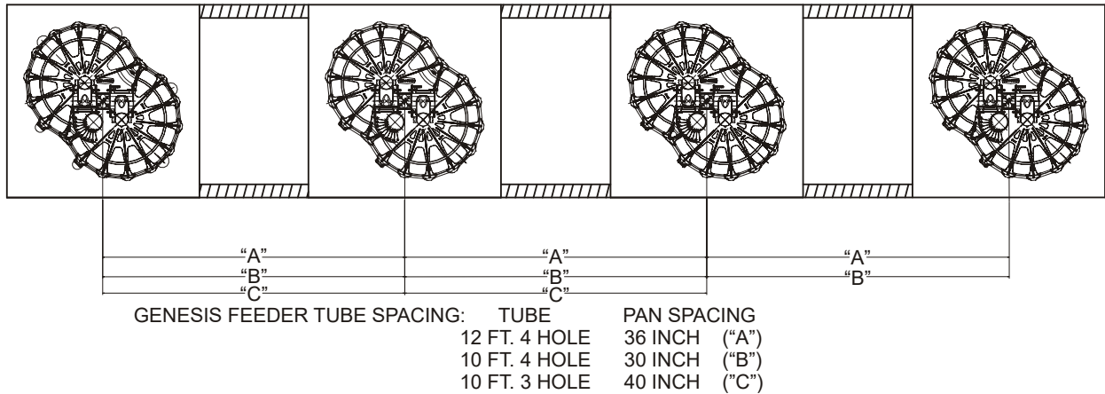
Figure 1. Pan Spacing
