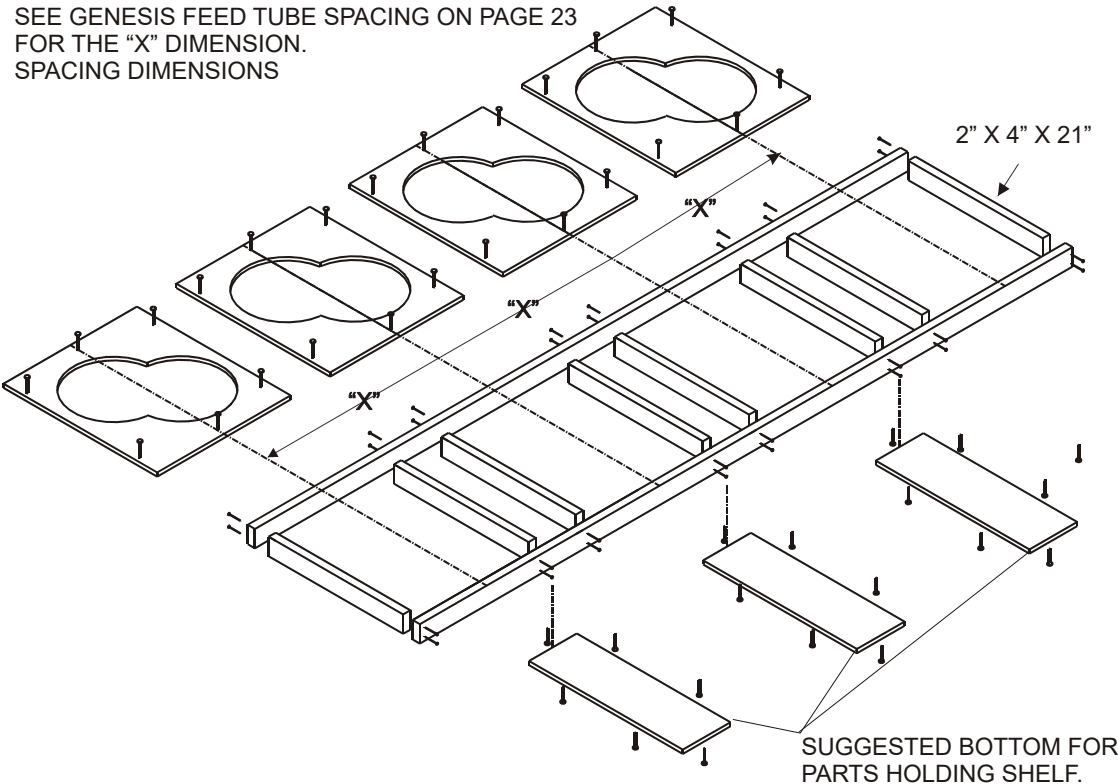
Figure 36. Feeder Pan and Tube Assembly Fixture Construction
