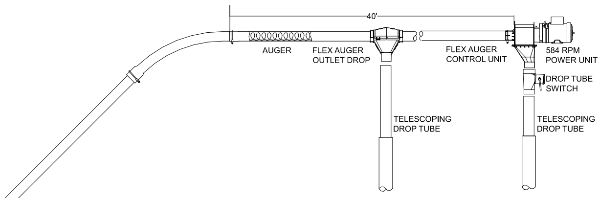
SAMPLE FLEX-AUGER LAYOUT REFERENCE ONLY
