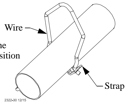
Figure 52. Hanger Installation
