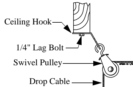
Figure 10. Wood Truss Ceiling Bracket and Pulley Installation
