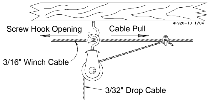
Figure 6. Screw Hook Installation
