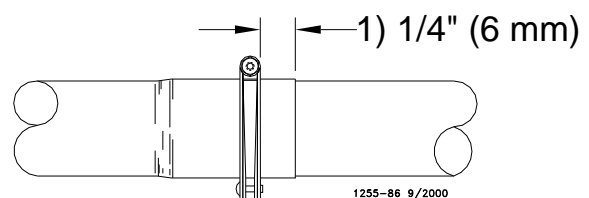
Figure 55. Tube Clamp Installation
