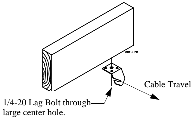
Figure 10. Wood Truss Ceiling Bracket and Pulley Installation
