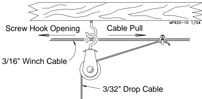
Figure 17. Drop Installation
