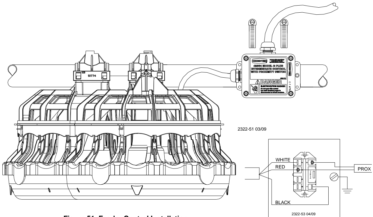
Figure 51. Feeder Control Installation
