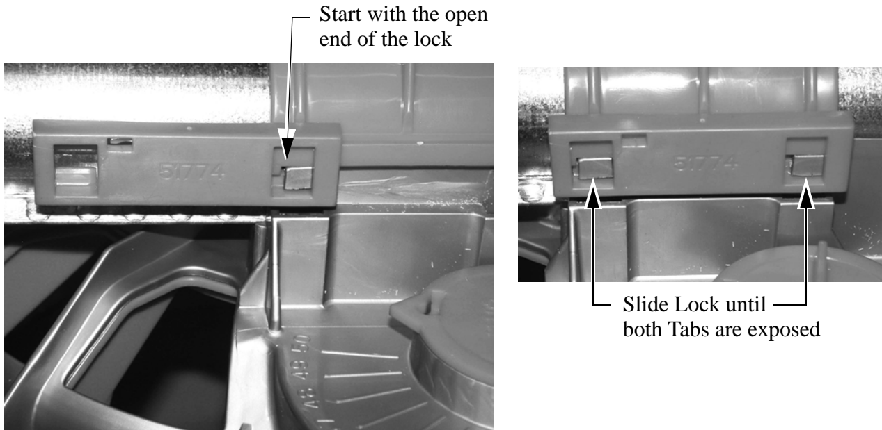
Figure 32. Slide Locks
