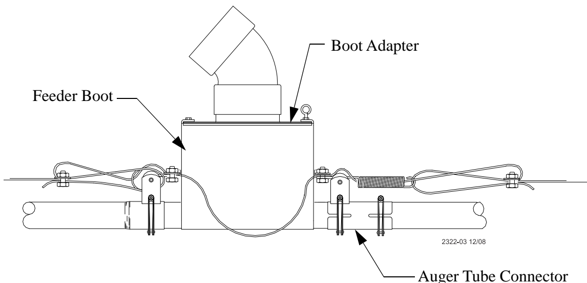
Figure 47. Elbow Assembly
