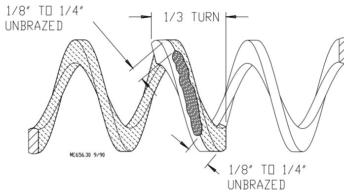
Figure 67. Brazing
