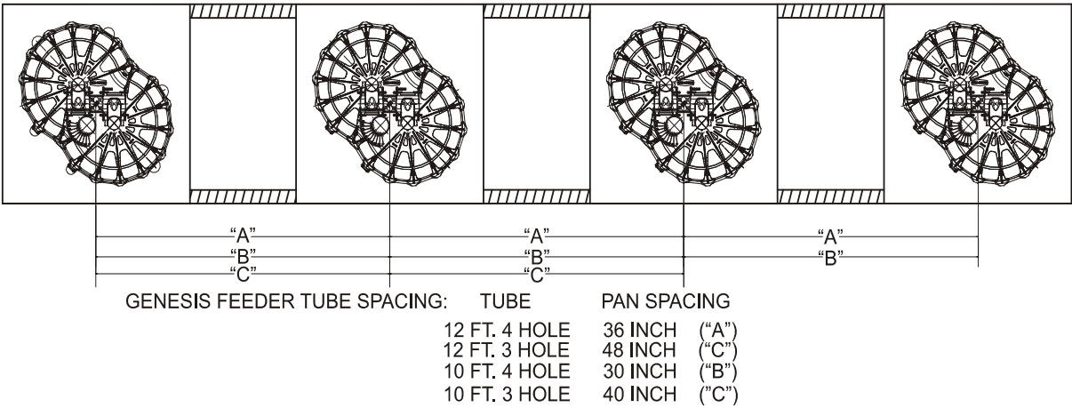
Figure 39. Pan Spacing
