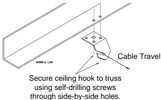
Figure 7. Narrow Steel Truss Ceiling Bracket Installation
