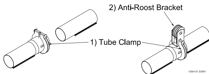
Figure 54. Tube Clamp and Clamp/Anti-Roost Bracket
