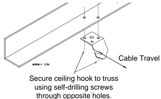
Figure 8. Steel Truss Ceiling Bracket Installation
