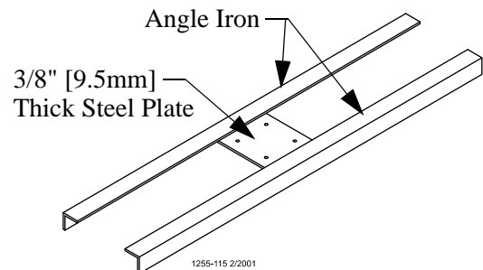
Figure 11. Optional Power Lift Winch Support detail
