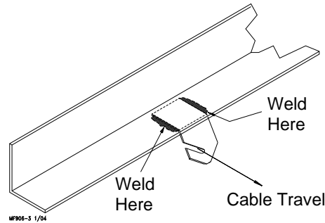
Figure 9. Welded Steel Truss Ceiling Bracket Installation
