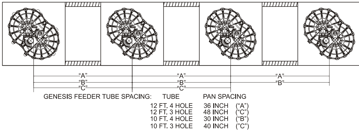
Figure 26. Pan Spacing
