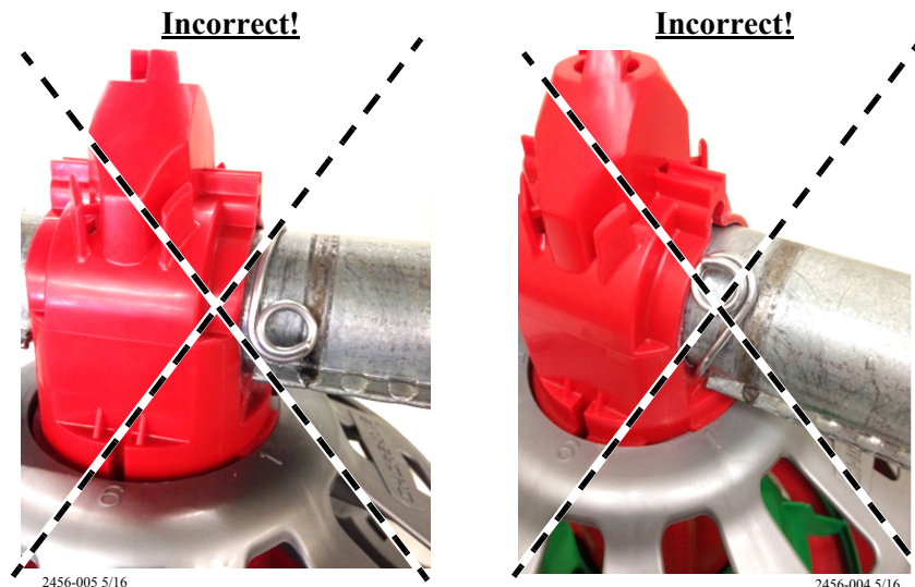
Figure 2. Incorrect installation
