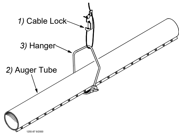
Figure 27. Hanger Installation
