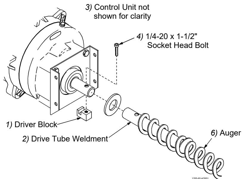
Figure 32. Auger Driver Components
