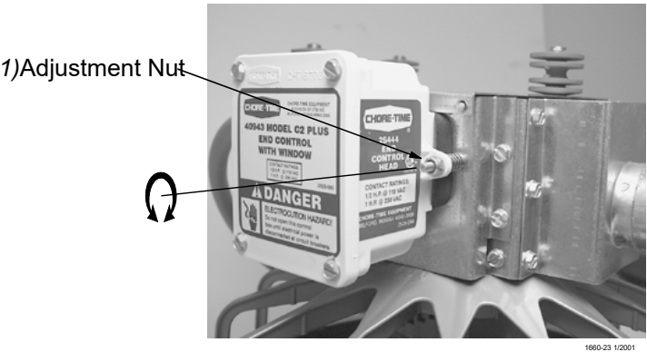
Figure 57.Switch Adjustment
