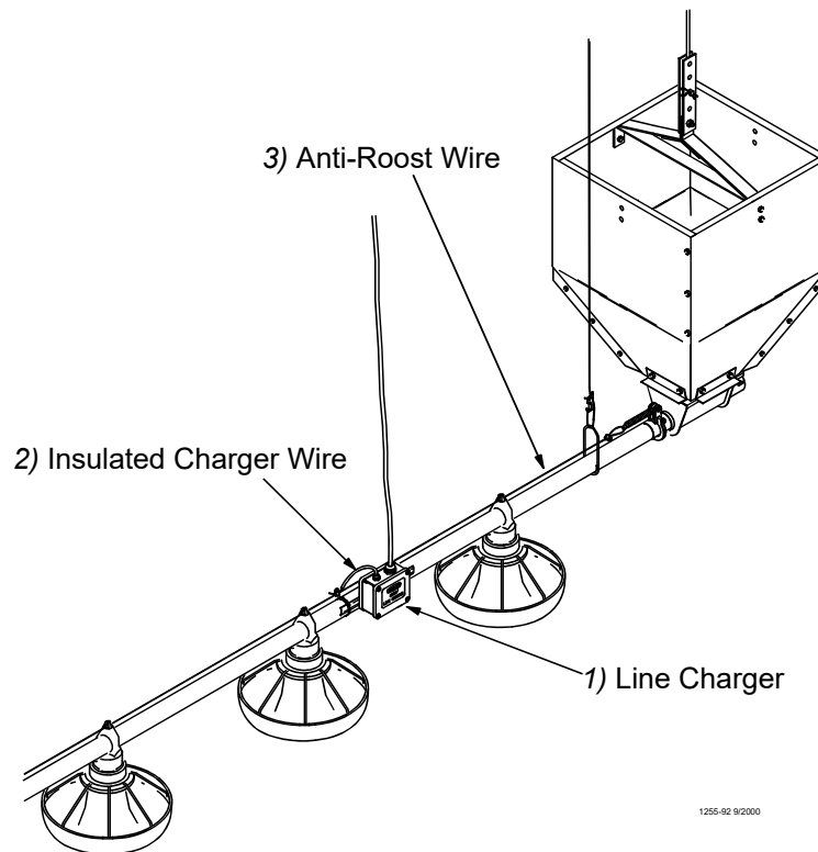
Figure 55. Line Charger Installation
