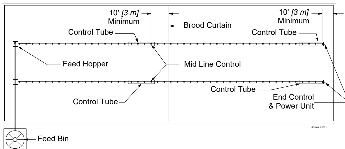
Figure 61. Component location diagram for systems over 400 feet [122 m]. (Top View).
