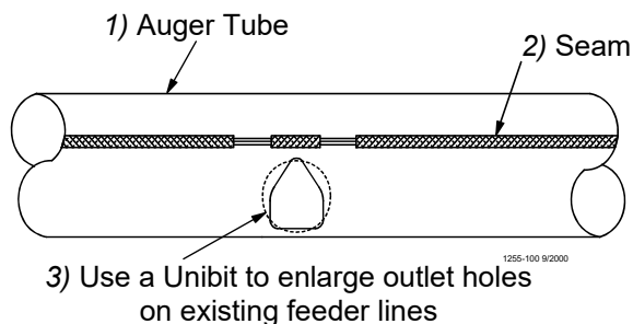
Figure 47. Enlarging Outlet Holes
