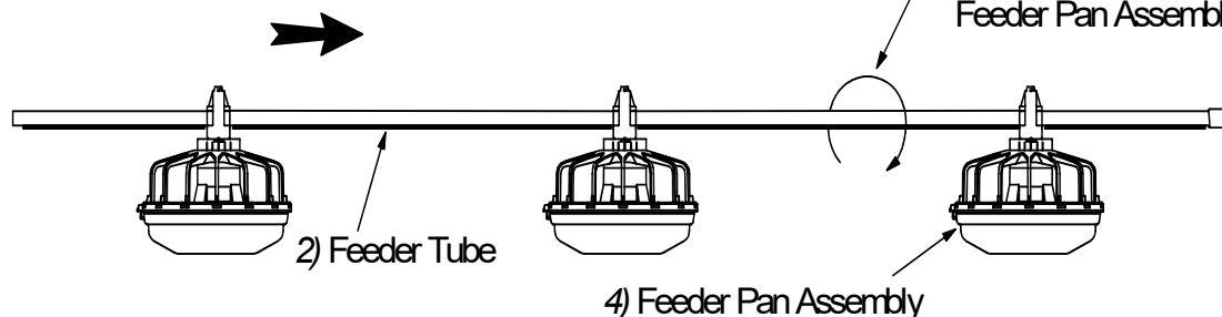
Figure 22. Assemble Feeders on tubes
