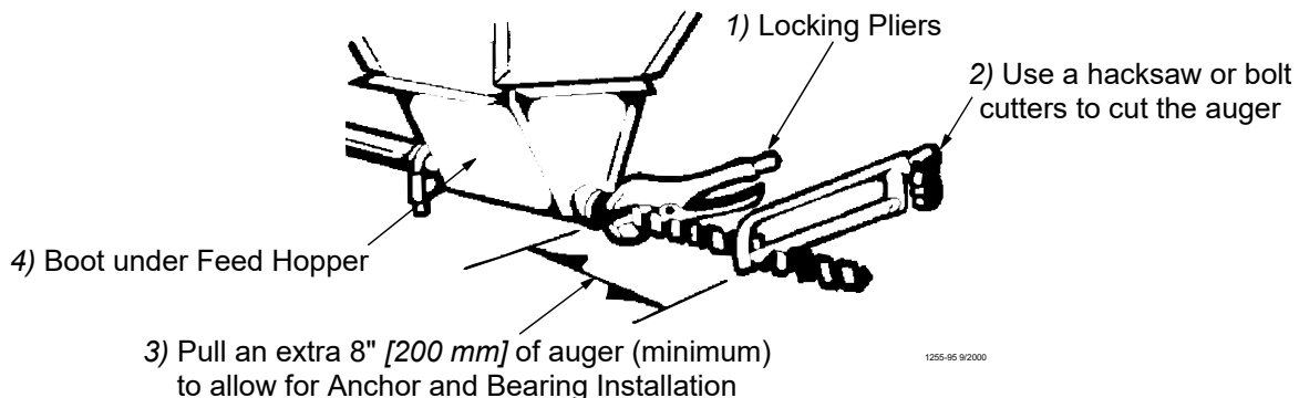
Figure 36. Cut Auger with required stretch
