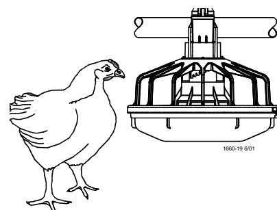
Figure 64. Feeder Pan Assembly height adjustment
