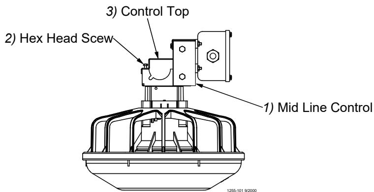
Figure 48. Mid-Line Control Installation
