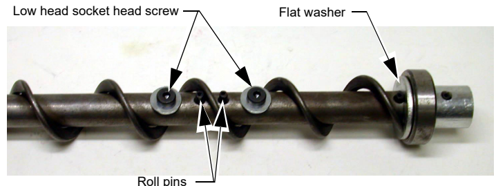
Figure 59. Auger and Anchor Bearing Connection
