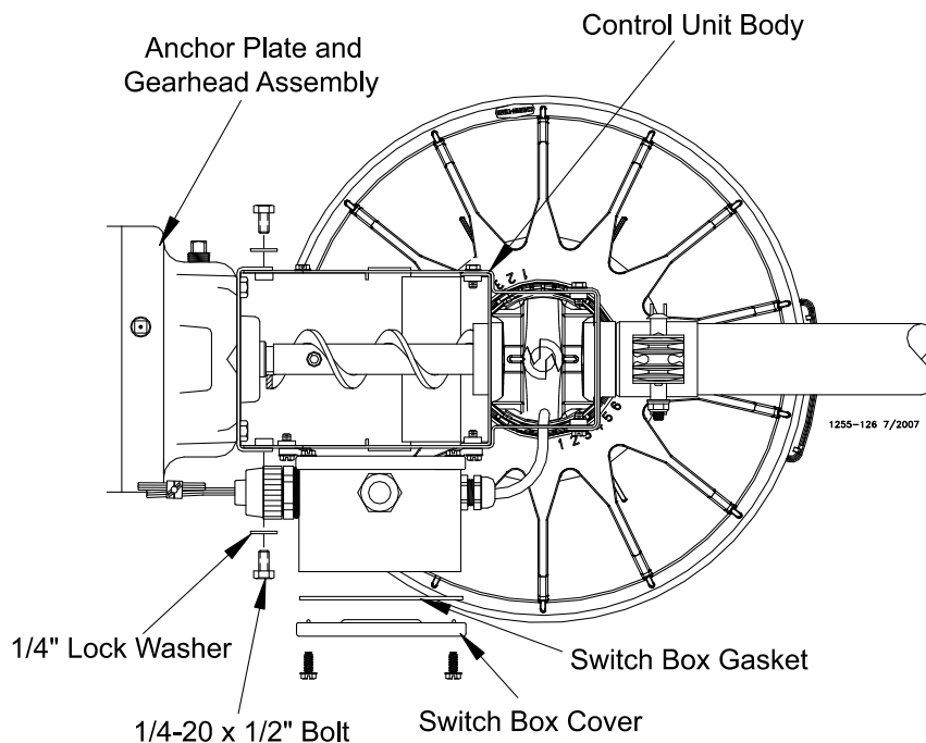
Figure 39. Attaching the Anchor Plate and Gearhead Assembly to the Control Unit Body
