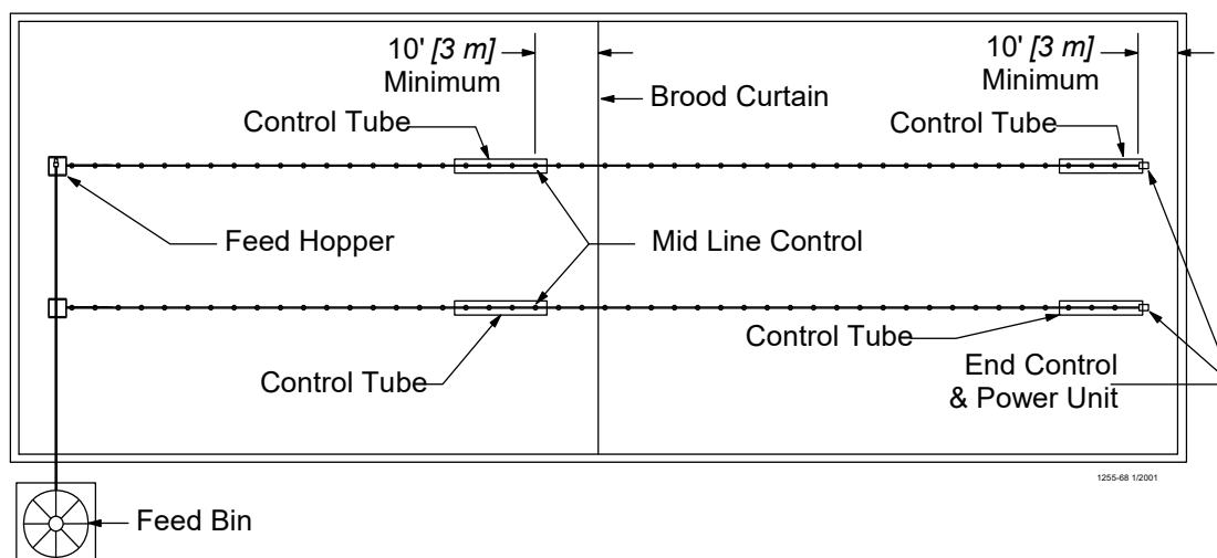
Figure 62. Component location diagram for systems up to 400 feet [122 m]. (Top View).
