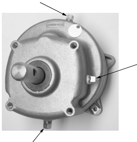
Figure 56. Gearhead Maintenance
