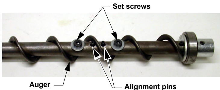
Figure 43. Auger and Anchor Bearing Connection
