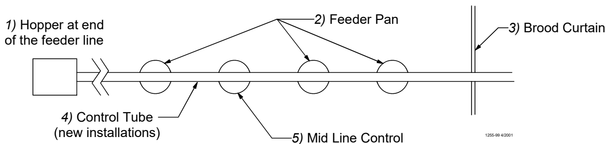
Figure 46. Mid-Line Control Location Diagram
