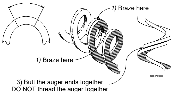
Figure 44. Auger Brazing
