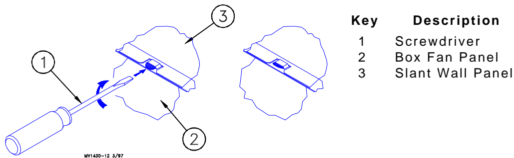
Figure 8. Slant Wall Lock Tab.
