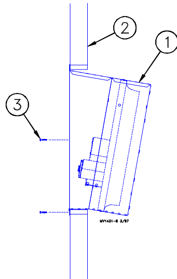
Figure 10. Fan installation (side view).
