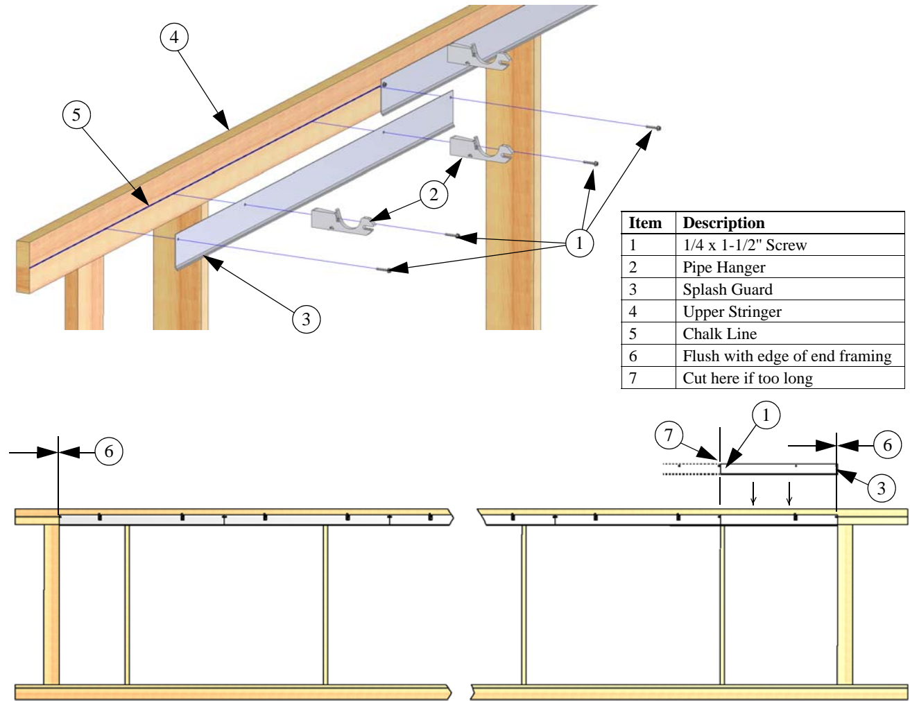
Figure 4. Pipe Support and Splash Guard Installation
