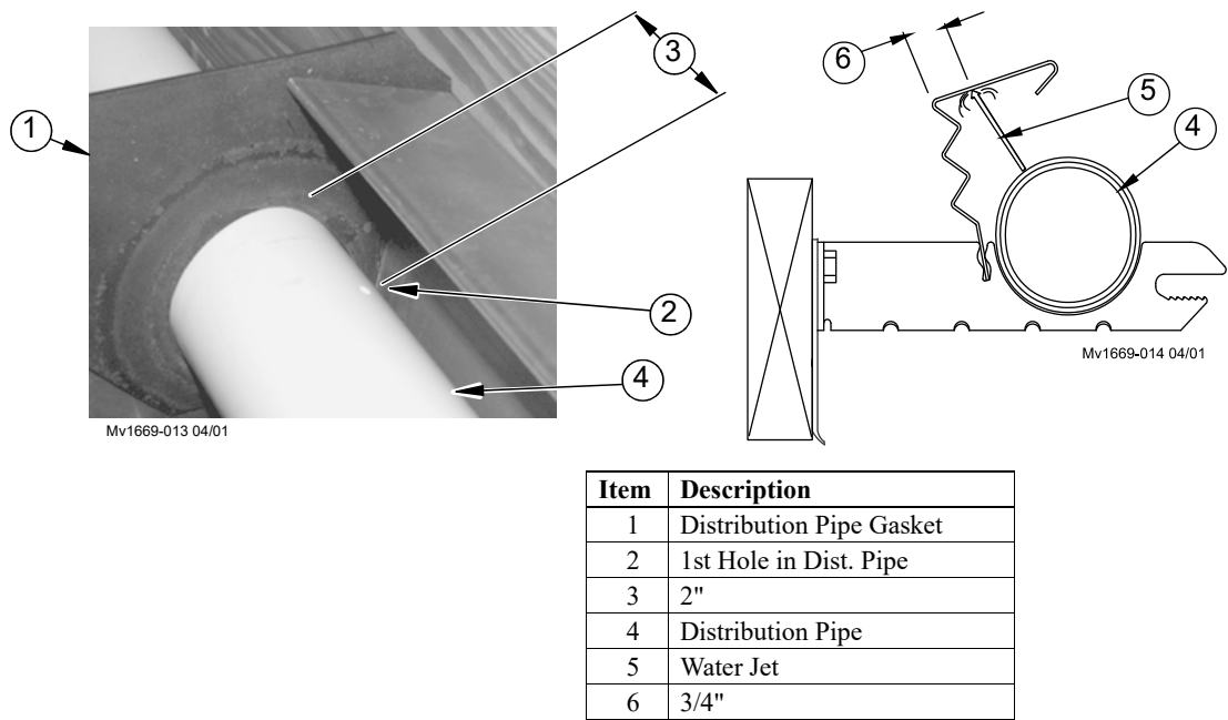
Figure 22.Orientating the Distribution Pipe
