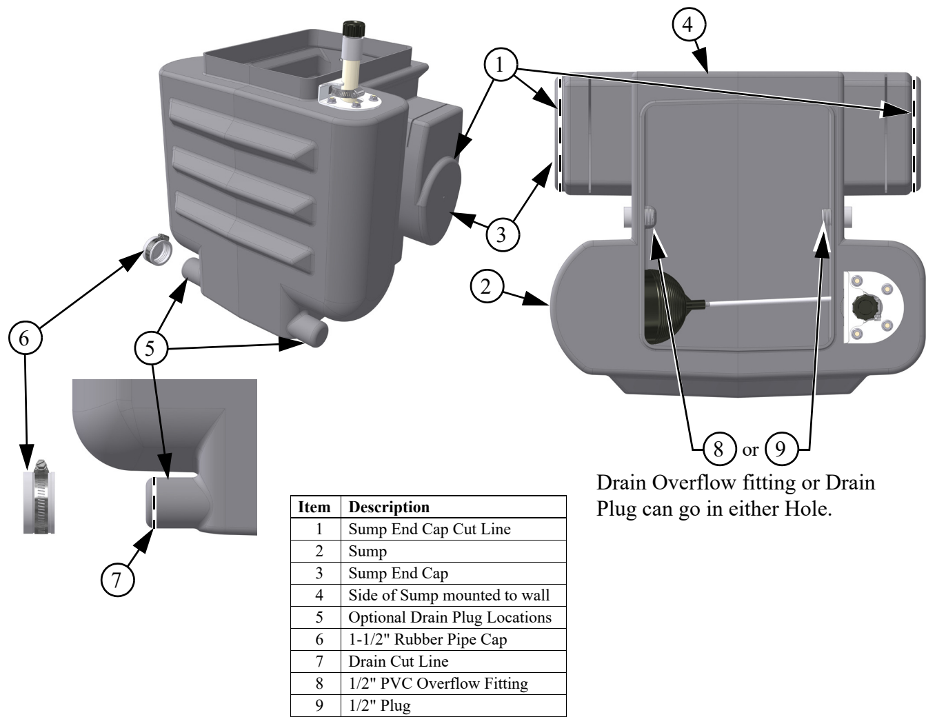
Figure 5.Sump Preparation
