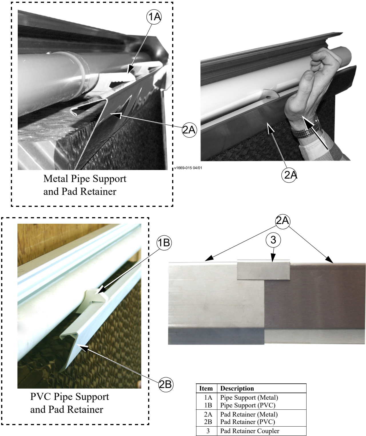
Figure 19. Pad Retainer Installation
