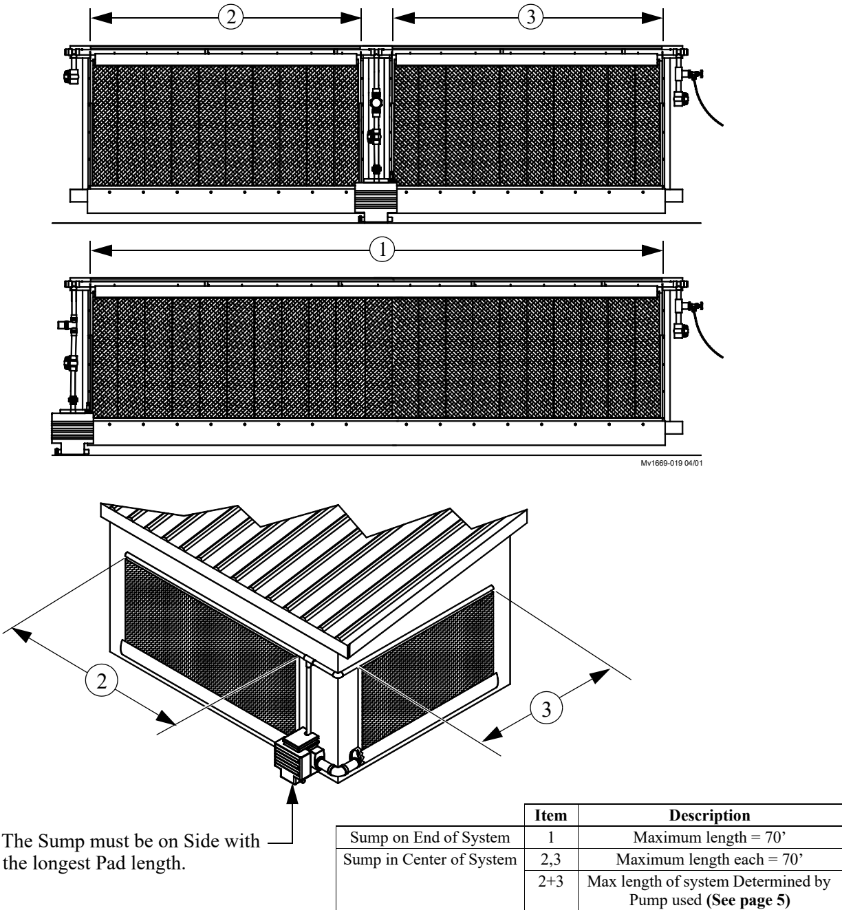
Figure 1.System Layout
