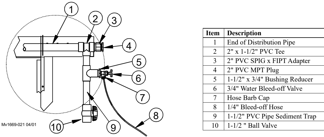
Figure 25.Sediment Trap Installation
