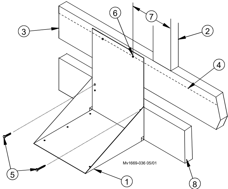
Figure 7.Sump Support Installation
