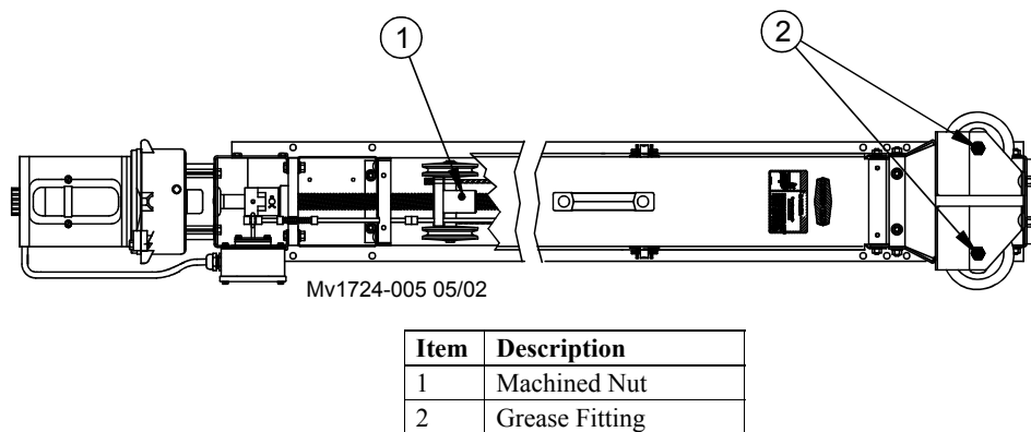
Figure 14. Swivel Top Linear-Lift Critical Grease Fitting Locations (horizontal wall mount view)
