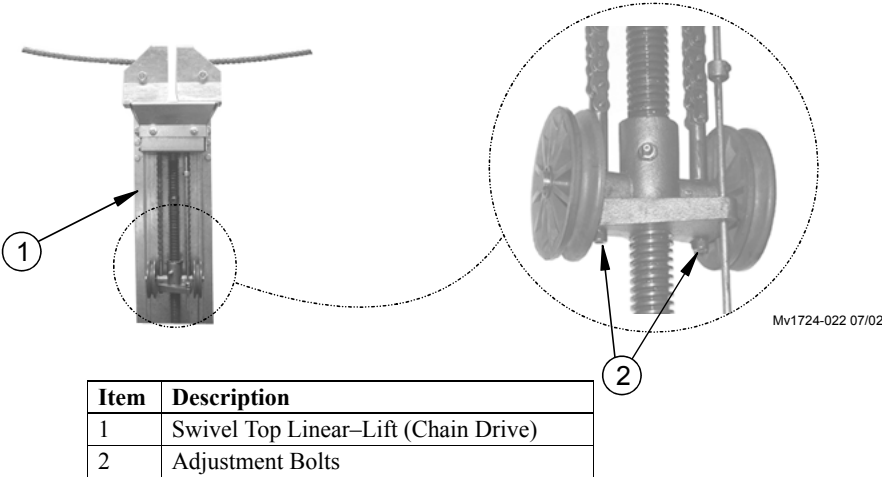
Figure 3. Bronze Nut Attachment Detail (Chain Drive)
