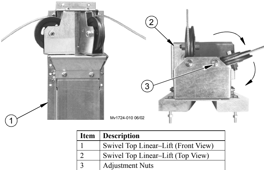
Figure 2. Swivel Top Pulley/Sprocket Angle Adjustment (Cable Version Shown)
