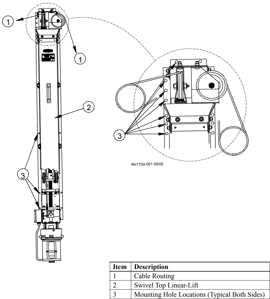
Figure 8. Swivel Top Linear-Lift Mounting Hole Locations
