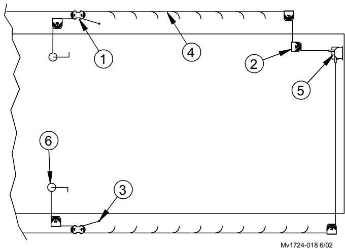
Figure 10. Wall Mounted (Corner) Swivel Top Linear-Lift pulling (2) curtains (top view)
