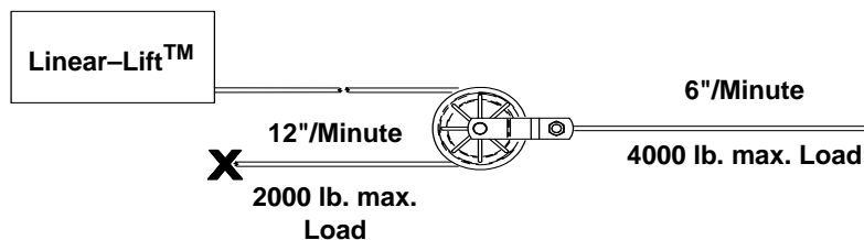
Figure 1. Cable/Pulley Combination
