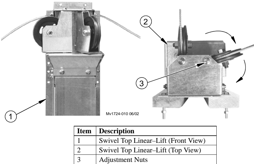
Figure 2. Swivel Top Pulley/Sprocket Angle Adjustment (Cable Version)
