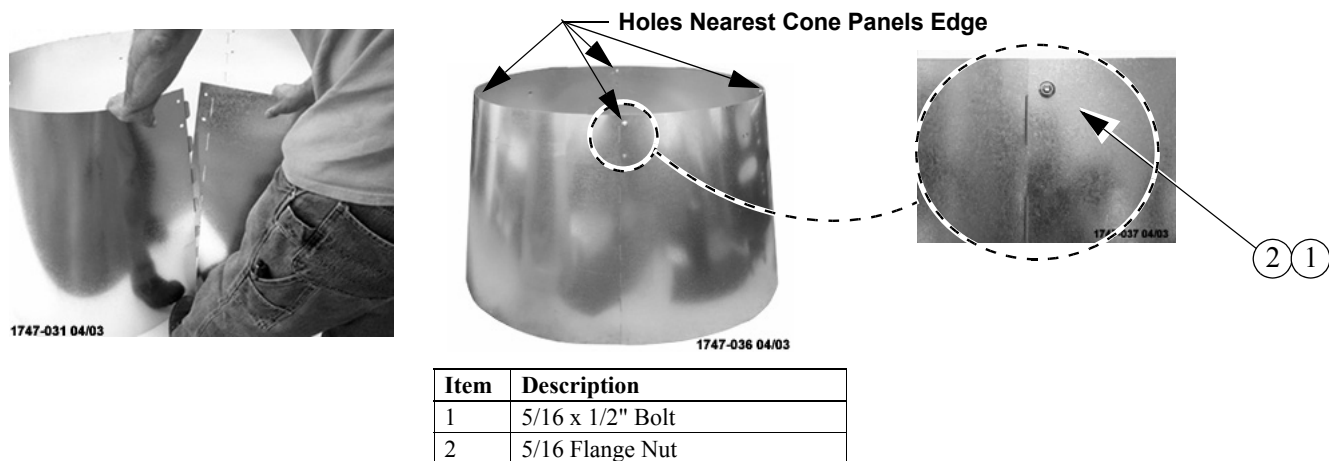
Figure 11. Bolting Cone Panels
