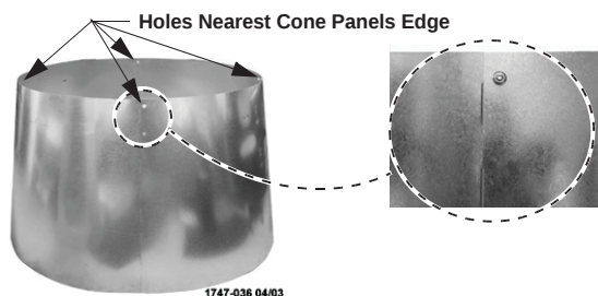
Figure 13. Assembling the Cone
