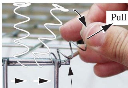
Slide Corner Wire C) Slide and Pull Spring over Corner Panel Wire.
