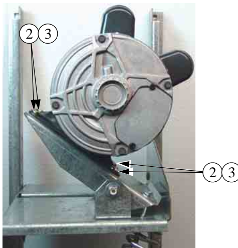
Figure 2. Remove Motor
