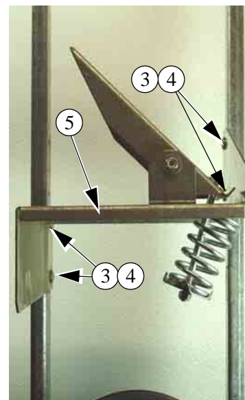
Figure 3. Remove Z Bracket
