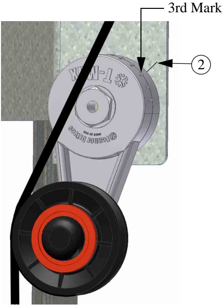
Figure 9. Correct Tensioner position
