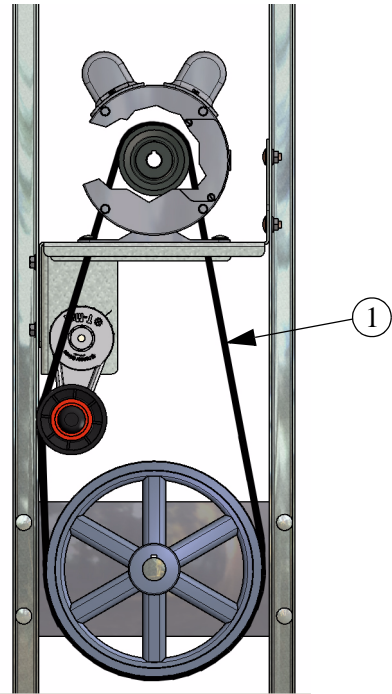
Figure 8. Installing new Belt
