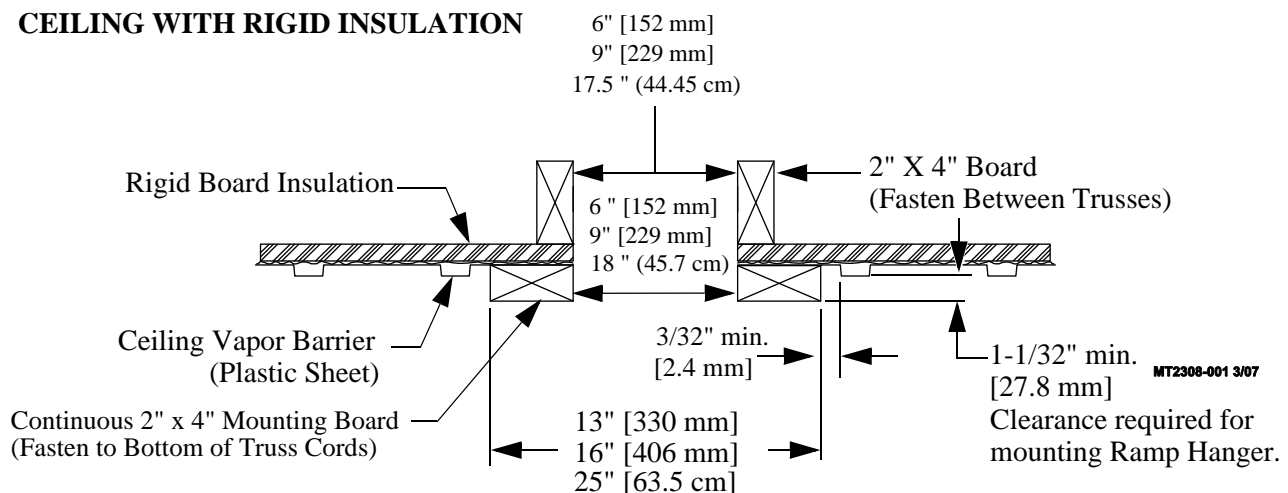
Figure 1. Ceiling Framing
