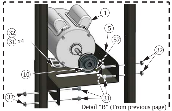
Detail "B" (From previous page)
