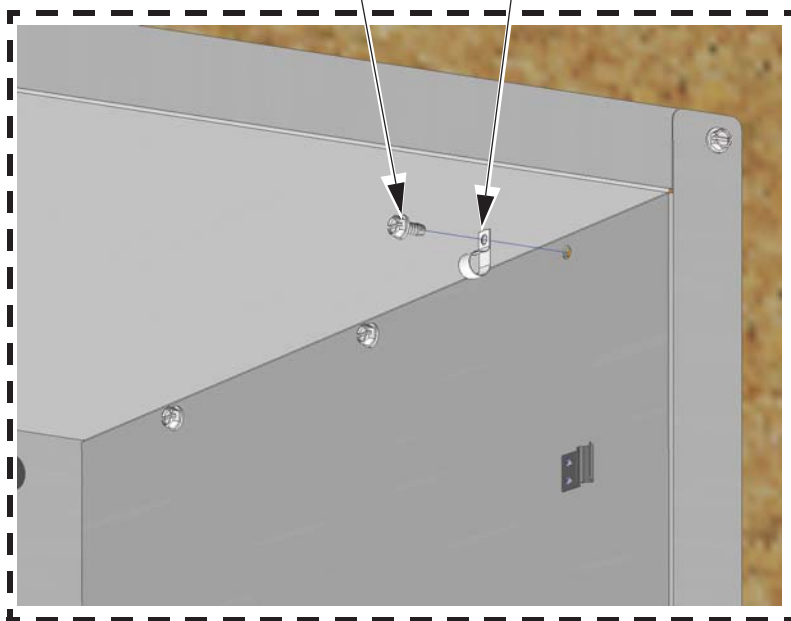
(54683) 1/4-20 x 1/2 Self Tapping Screw
