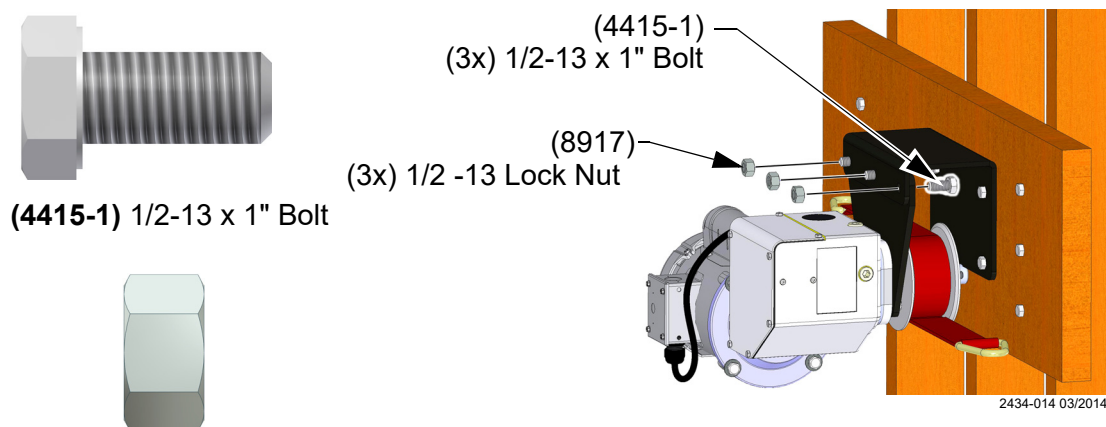
Figure 6. Attaching Winch to Wall Mount Bracket
