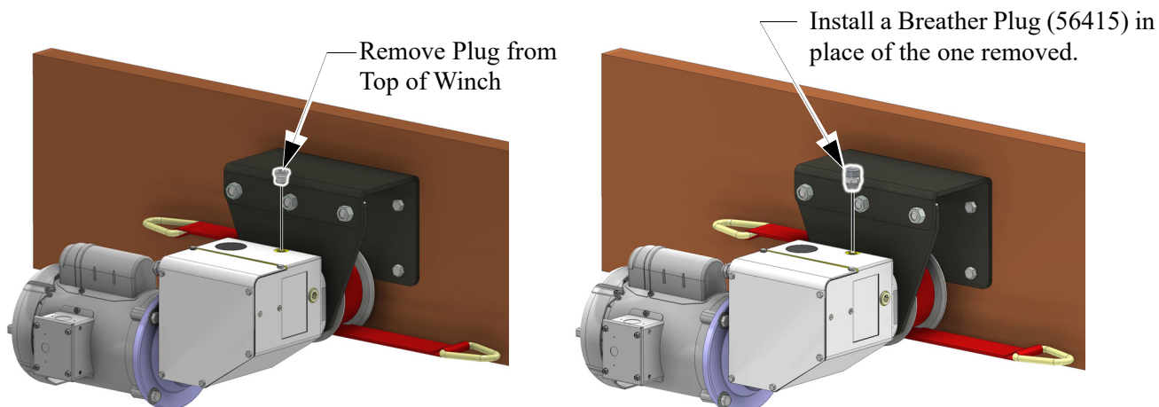
Figure 8. Installing Breather Plug
