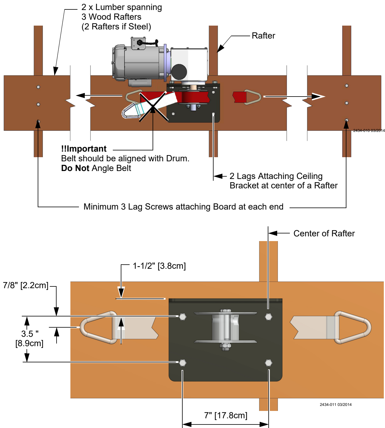
Figure 5.Ceiling Mounting Bracket
