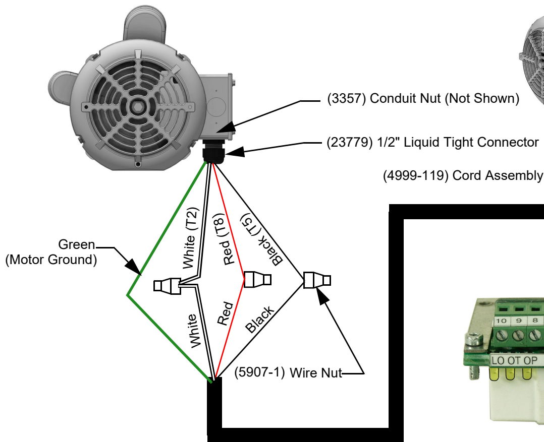
Figure 3. Motor Wiring
