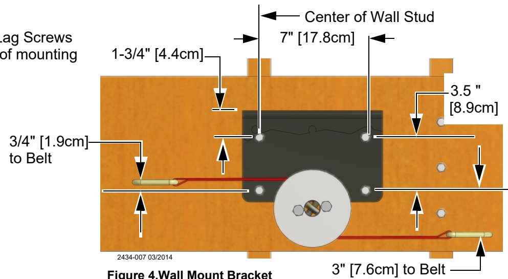
Figure 4. Wall Mount Bracket
