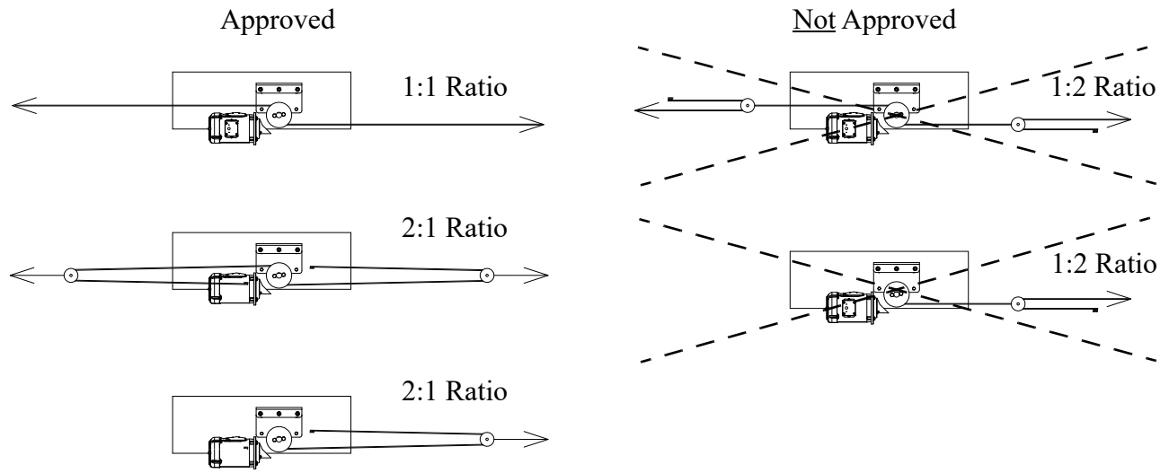
Figure 9.Proper Cabling
