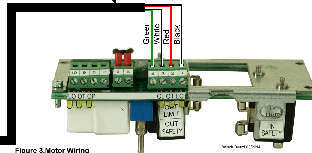
Figure 3. Motor Wiring
