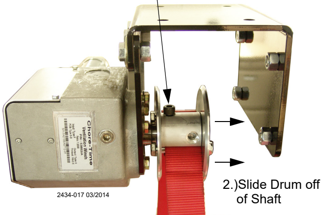
Figure 12. Removing Strap
