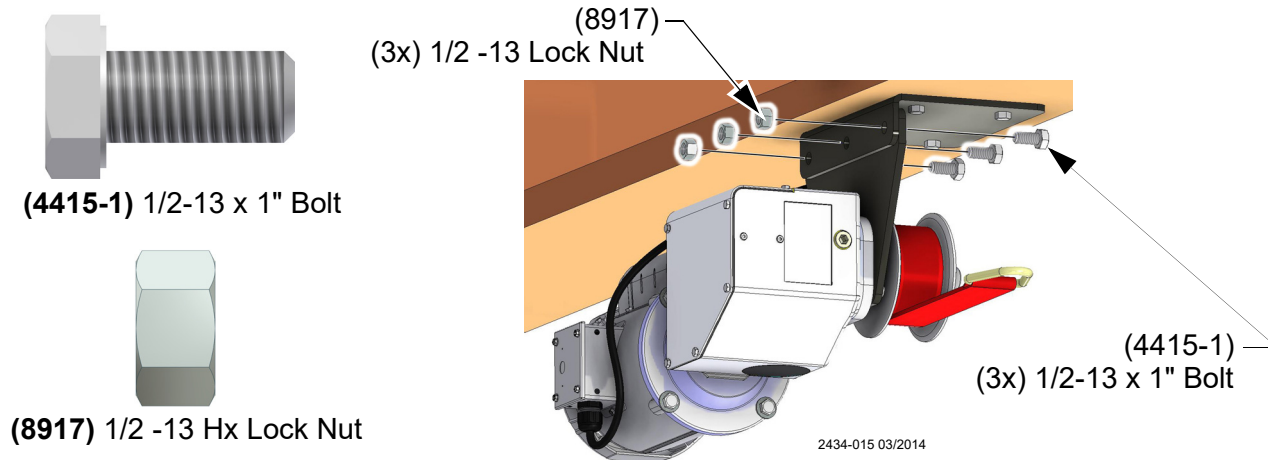
Figure 7. Attaching Winch to Ceiling Mount Bracket
