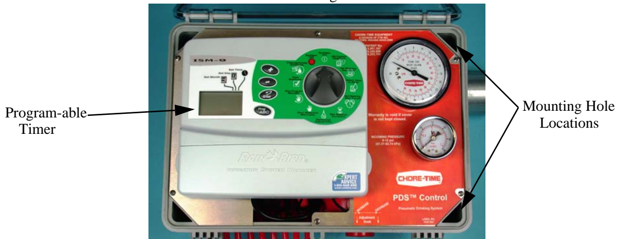
Figure 3. Mounting orientation
