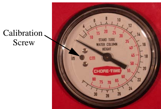
Figure 9. Water Column Gauge
