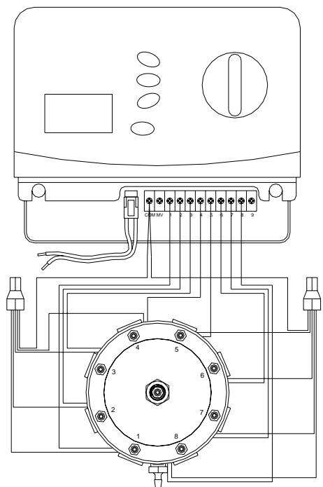
Figure 5. Internal Wiring
