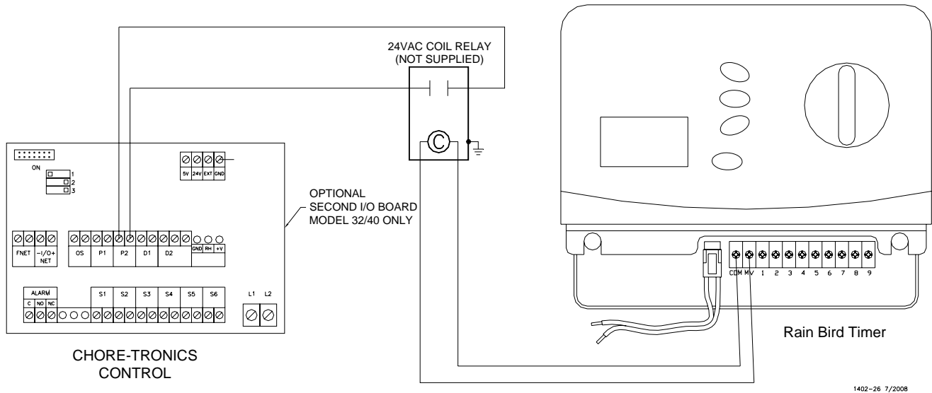
Figure 4. Rain Bird/Chore-Tronics Wiring
