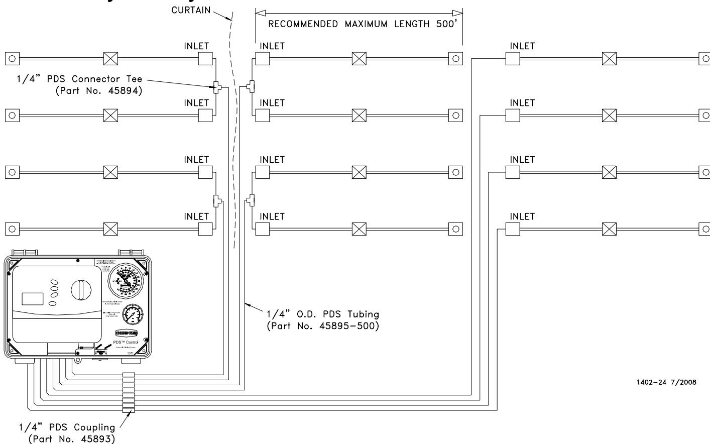
Figure 1. Broiler Layout
