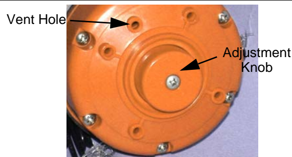
Figure 1. Vent Hole
