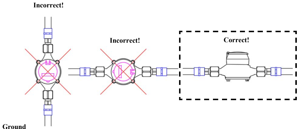
Figure 20. Water Meter Mounting
