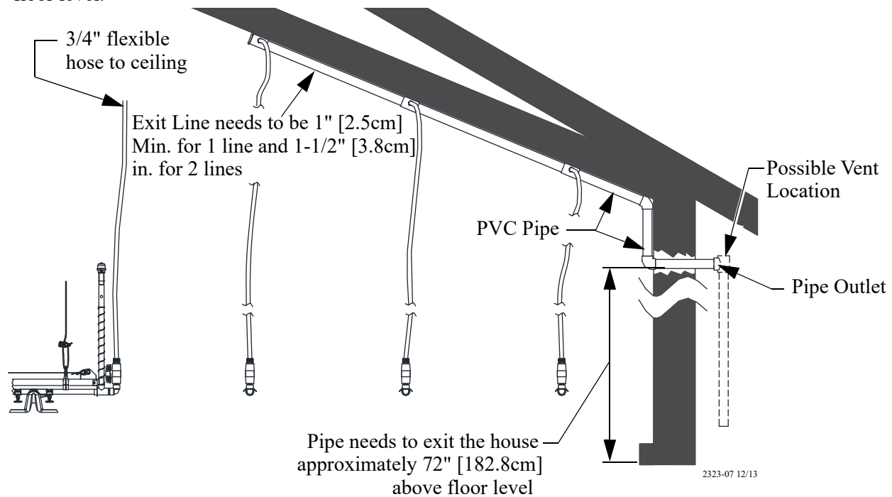
Figure 24. Anti-Roost Components
