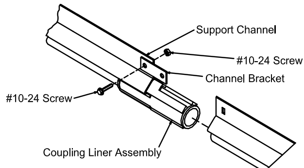
Figure 11. Securing the Water Line together
