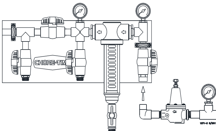
Figure 18. Optional Control Panels
