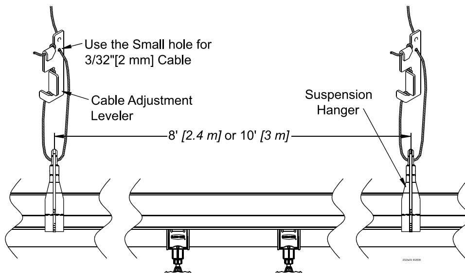
Figure 17. Suspend Water Lines
