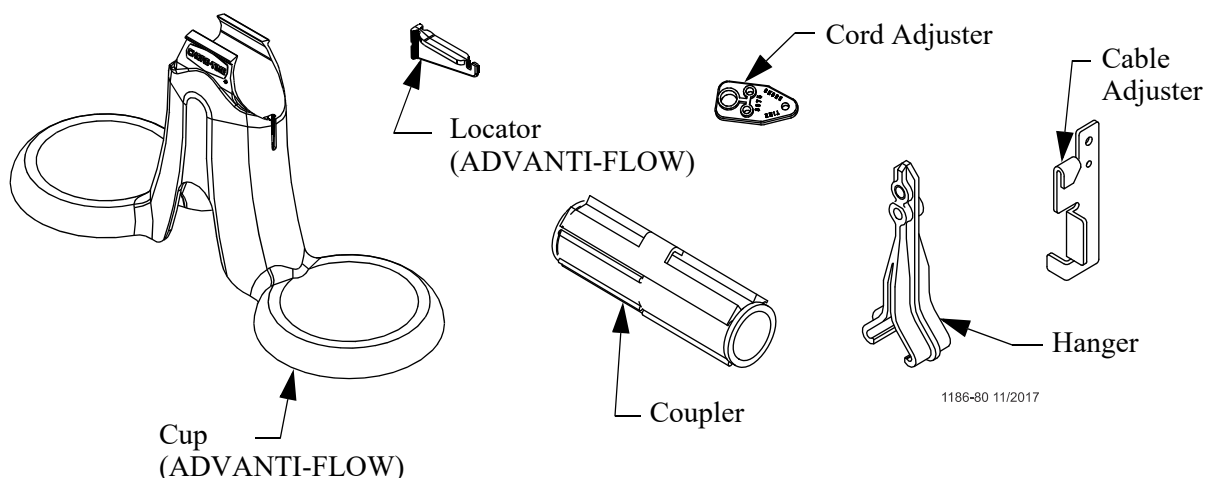
Figure 14. Nipple Waterer Components
