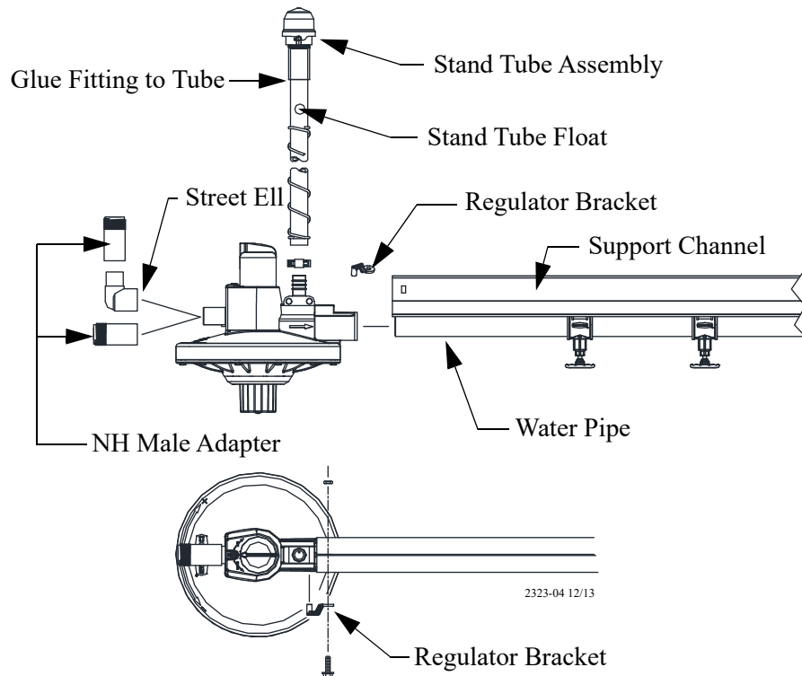
Figure 24. Regulator Assembly Components
