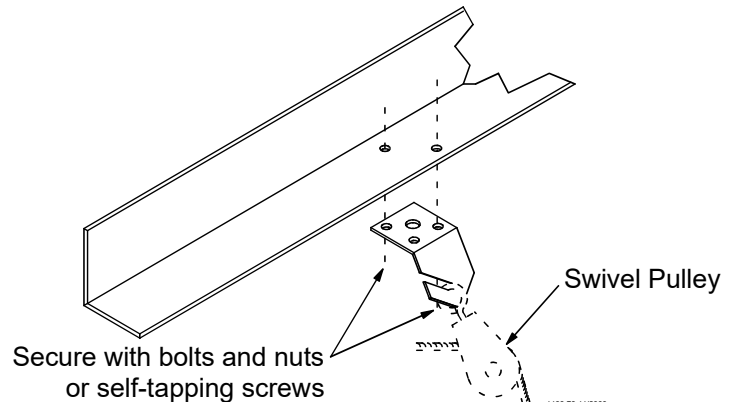
Figure 9. Ceiling Hook Installation
