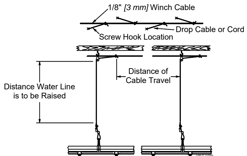
Figure 10. Offset the Screw/Ceiling Hooks
