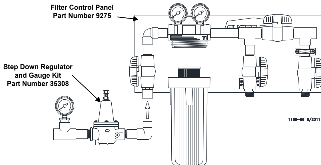
Figure 25. 9275 Control Panel
