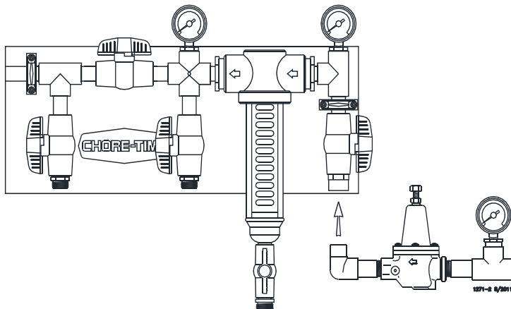
Figure 26. Optional Control Panels
