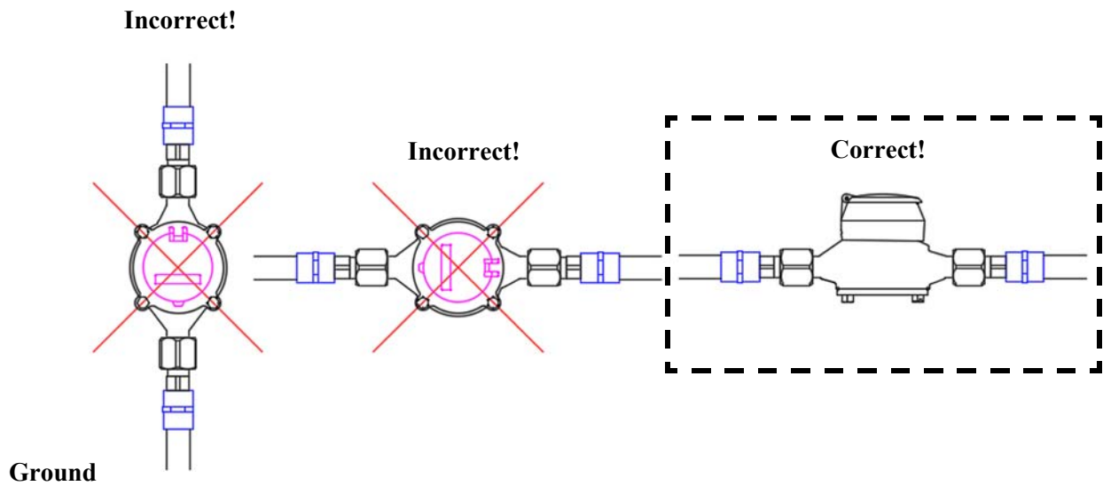
Figure 28. Water Meter Mounting
