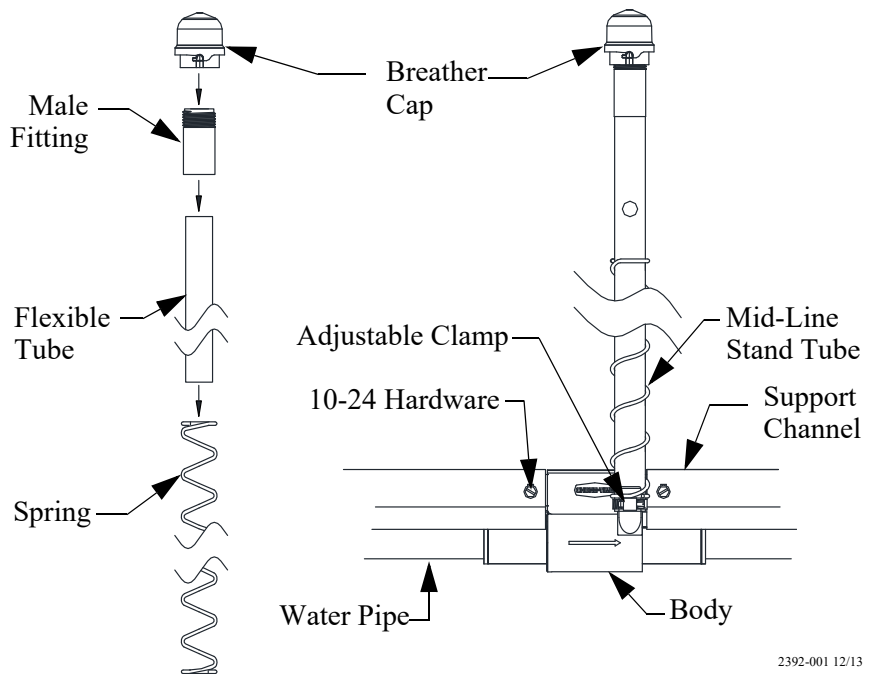
Figure 20. Mid Line Stand Tube Installation
