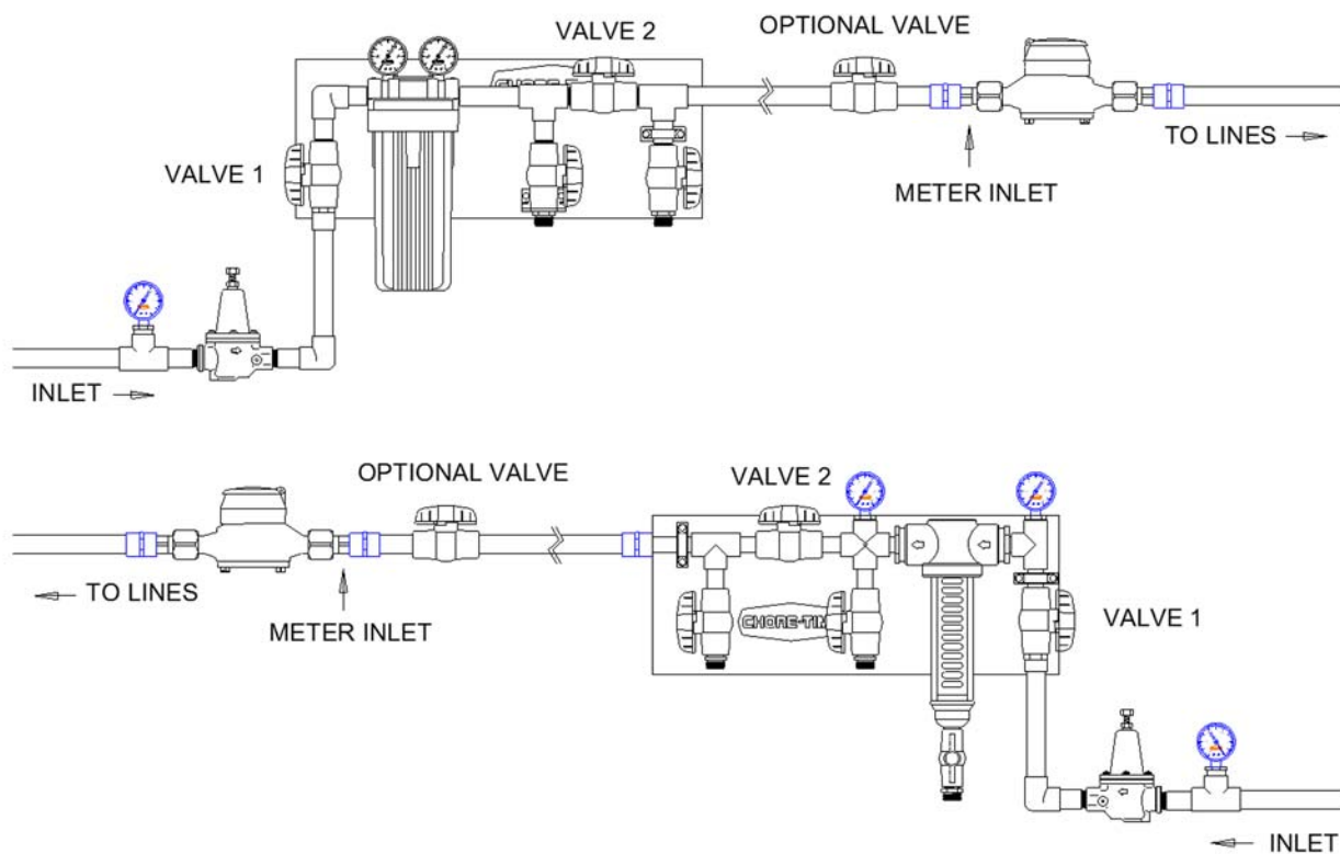
Figure 29. Water Meter Start Up
