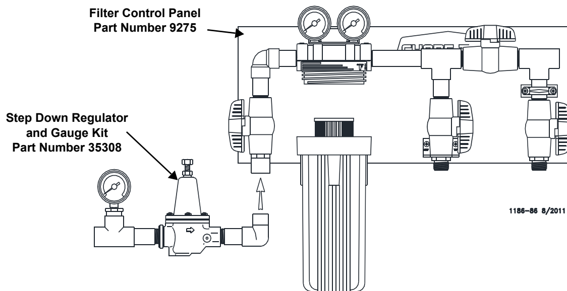
Figure 24. 9275 Control Panel
