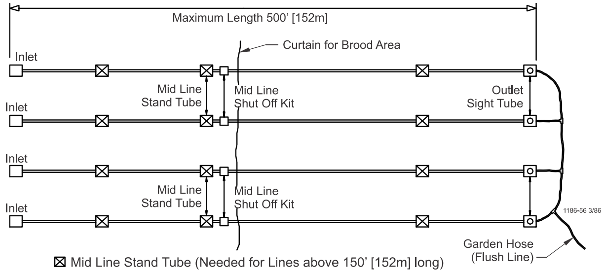
Figure 6. Alternate Layout #2 for RELIA-FLOW® and STEADI-FLOW®
