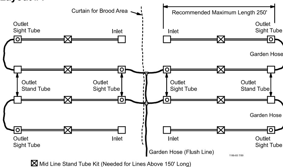
Figure 5. Alternate Layout for RELIA-FLOW® and STEADI-FLOW®
