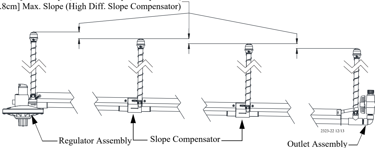
Figure 21. Slope Compensator Assembly Installation
