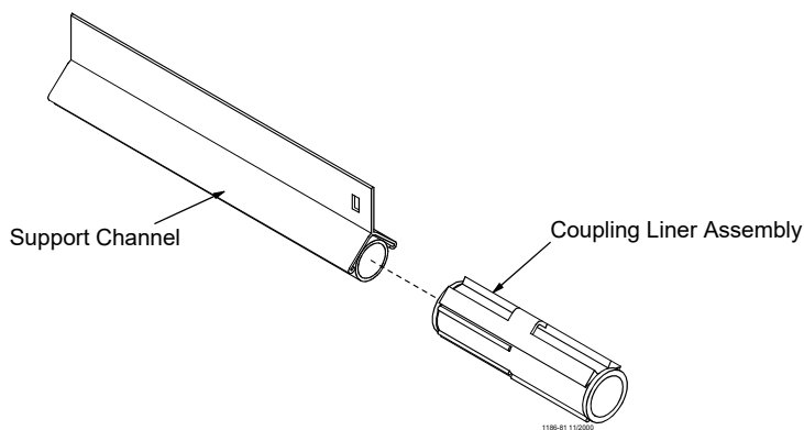
Figure 15. Coupling Liner Assembly Installation
