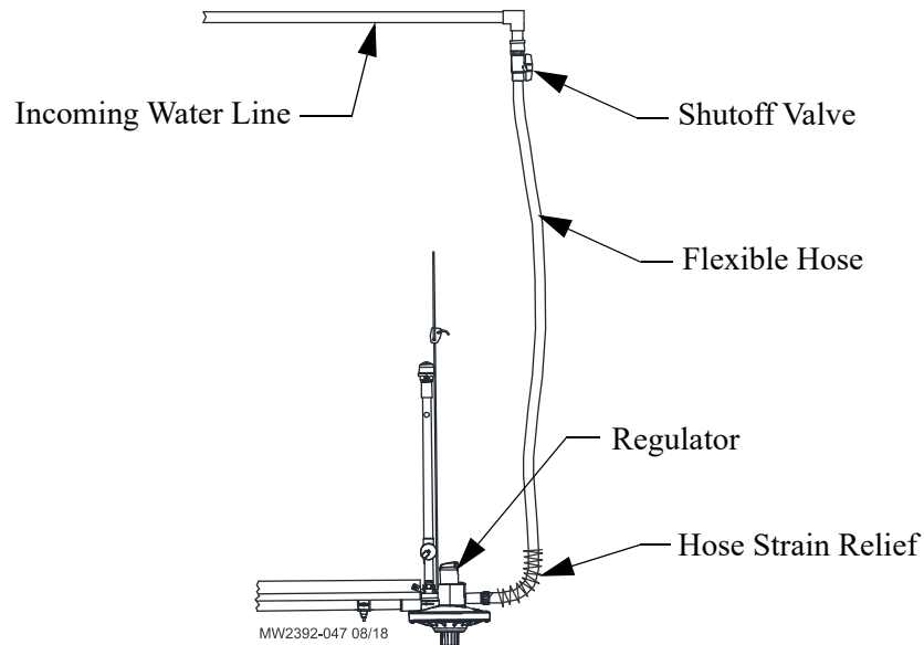
Figure 31.Incoming Water System
