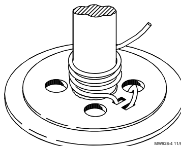
Figure 12. Cable Wrap on Drum
