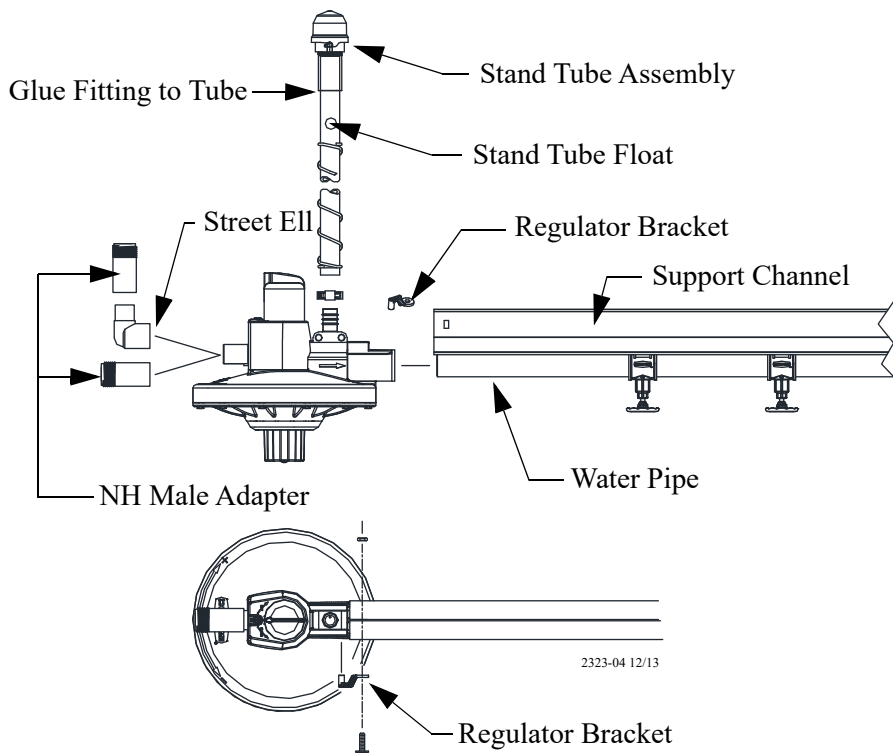
Figure 23. Regulator Assembly Components
