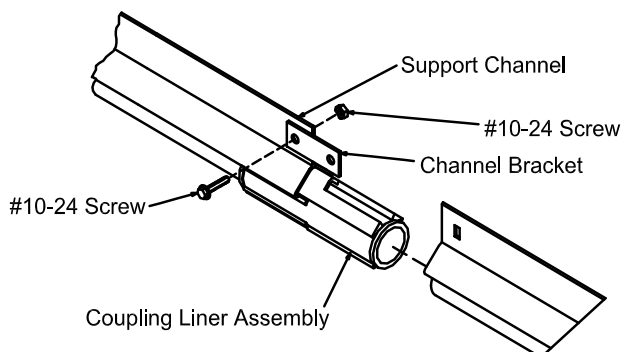
Figure 16. Securing the Water Line together
