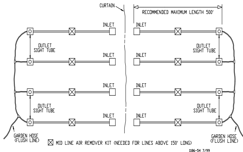
Figure 4. Preferred Layout for RELIA-FLOW® and STEADI-FLOW®
