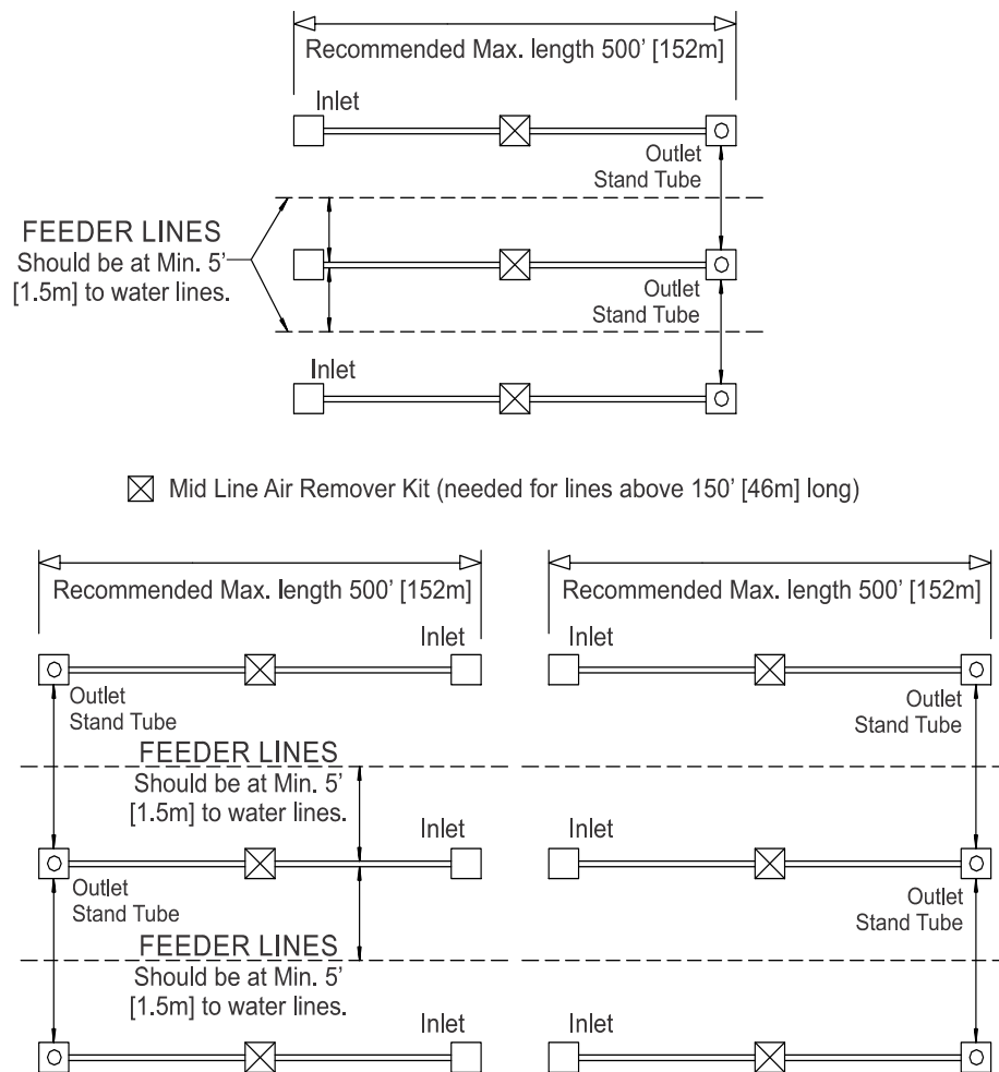
Figure 7. Preferred Layouts for ADVANTI-FLOW®
