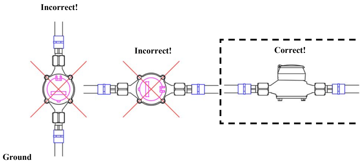
Figure 27. Water Meter Mounting
