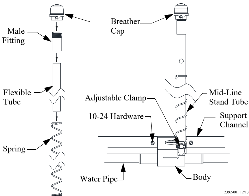
Figure 19. Mid Line Stand Tube Installation
