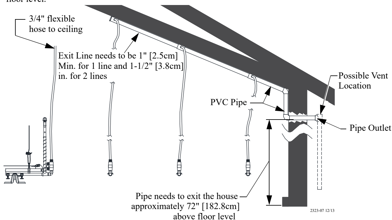
Figure 32. Flush System
