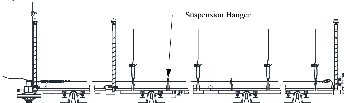
Figure 29. Regulator End Components
