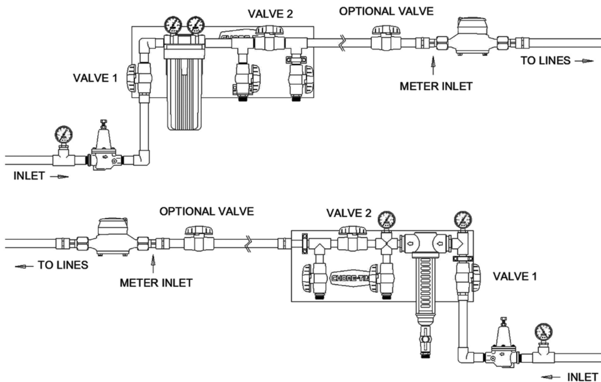
Figure 28. Water Meter Start Up
