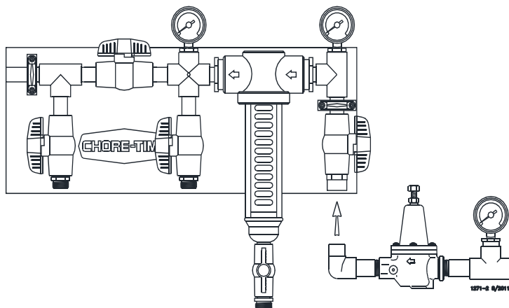
Figure 25. Optional Control Panels
