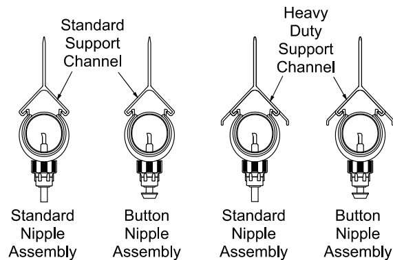
Figure 2.VariouS STEADI-FLOW® Drinker Styles
