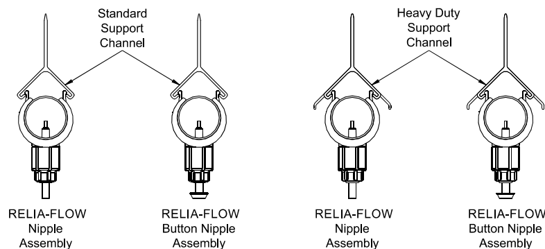
Figure 3.VariouS RELIA-FLOW® Drinker Styles
