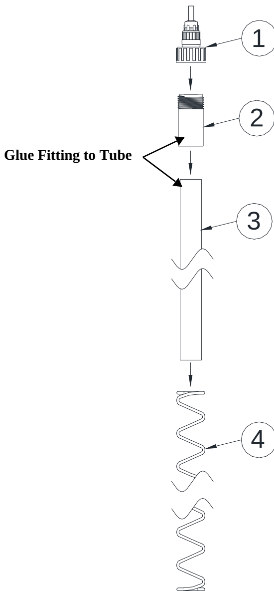
Figure 1. Stand Tube Assembly
