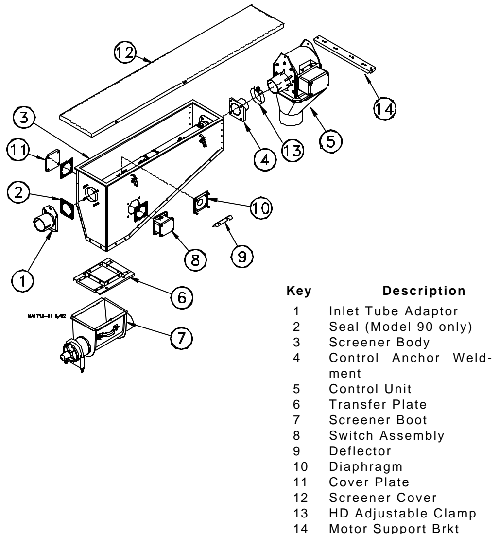
Figure 7. Model 90 and Model 108 Screener Assembly Procedure.
