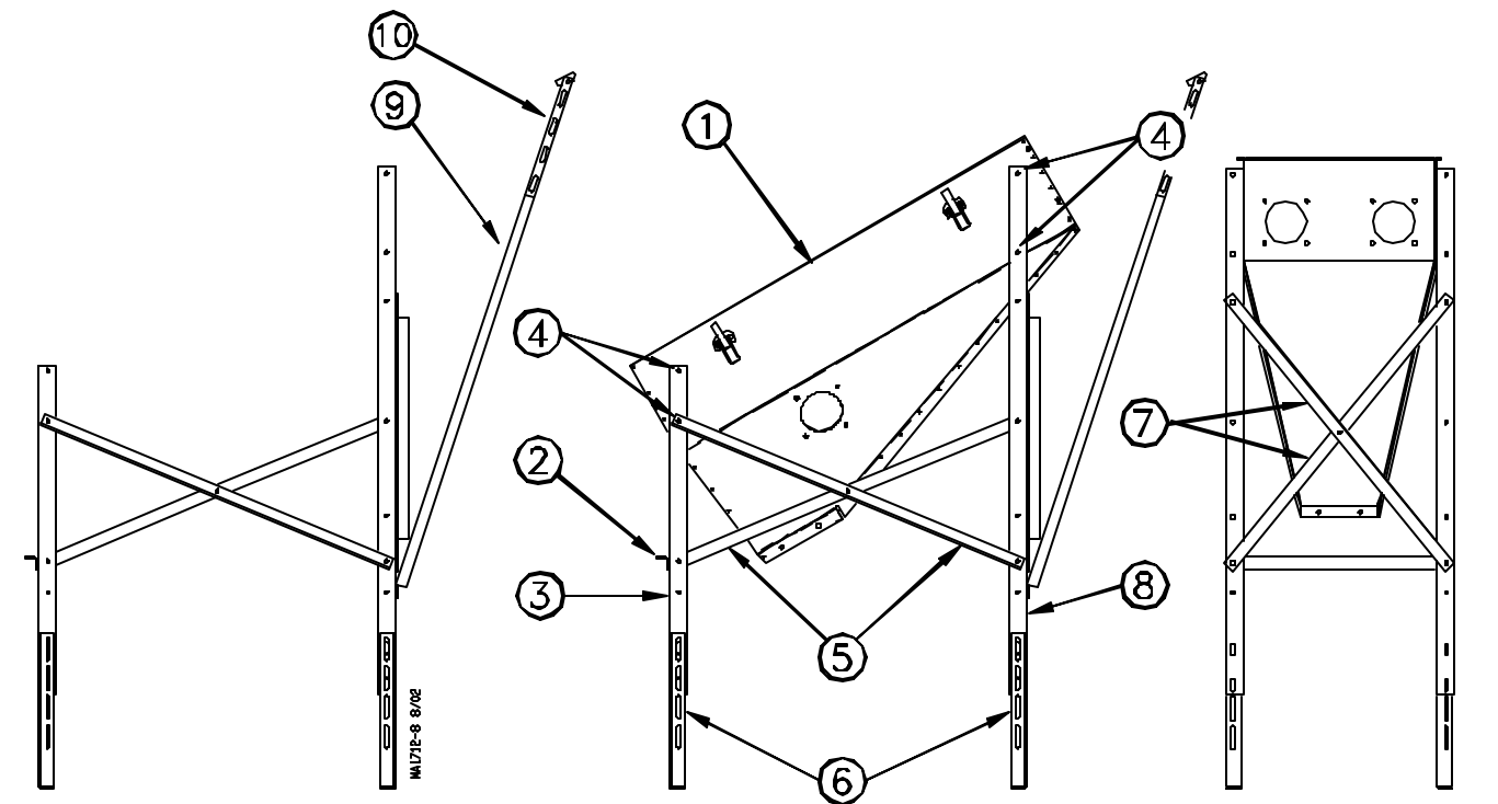
Framing Assembled (Side View)
