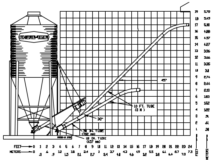
Figure 5. 30° Bin Boot with Feed Screener Boot in-line.
