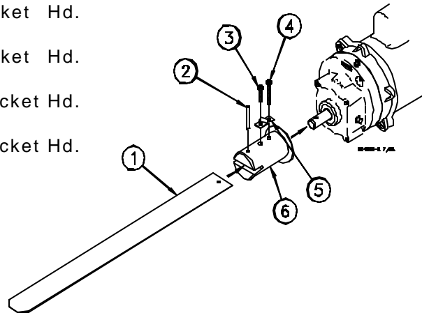
Figure 14. Model 90 & 108 Driver Components
