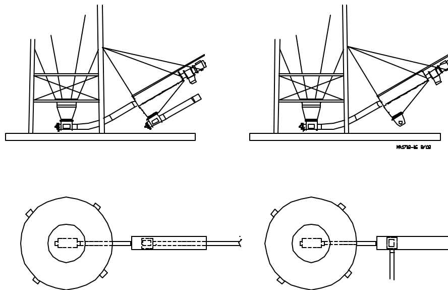
Figure 2. Model 90 & 108 Feed Screener Layout Diagram
