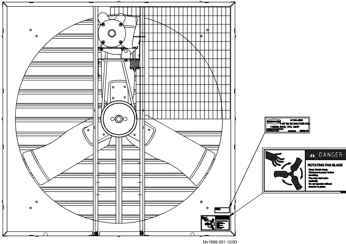
Figure 1. Decal Placement
