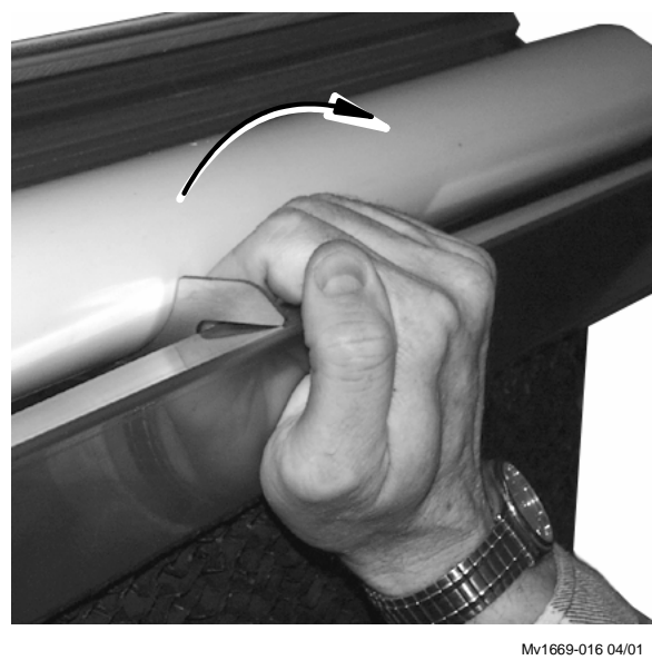
Figure 21. Removing the Pad Retainer
