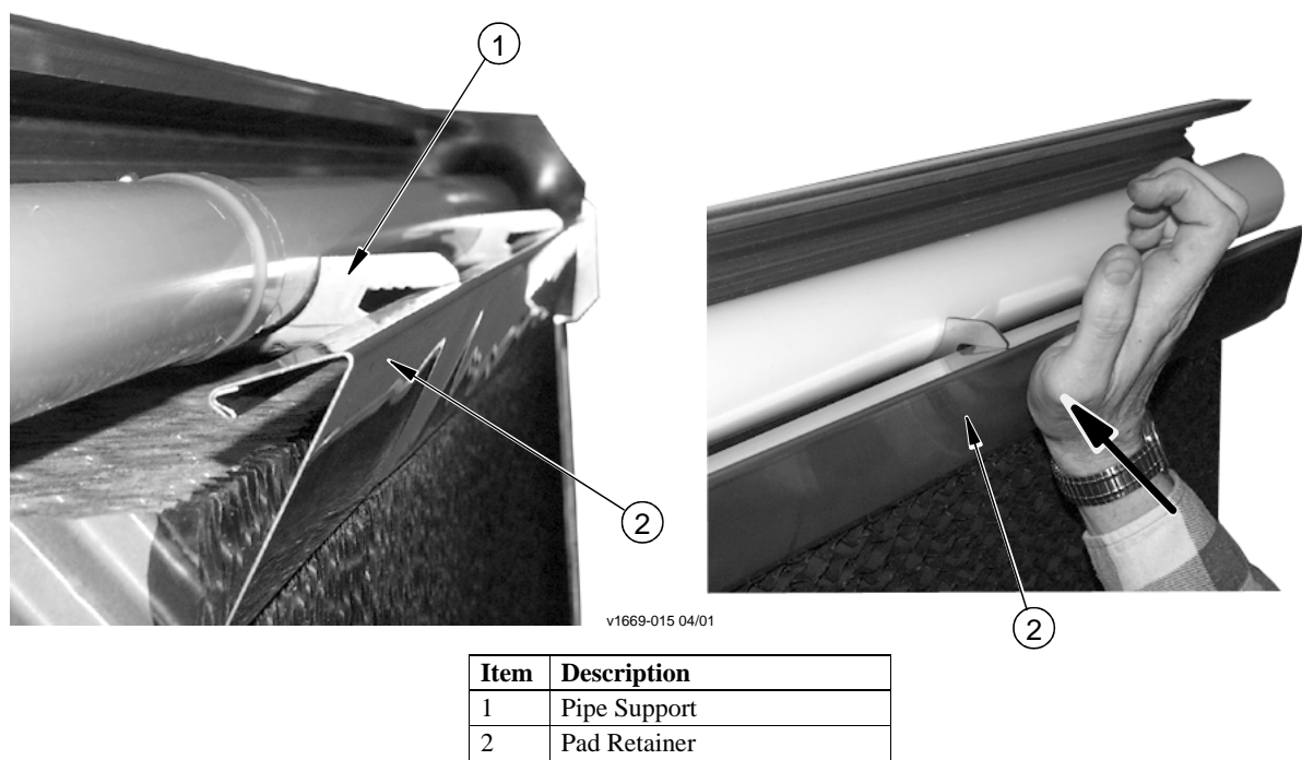
Figure 20. Pad Retainer Installation
