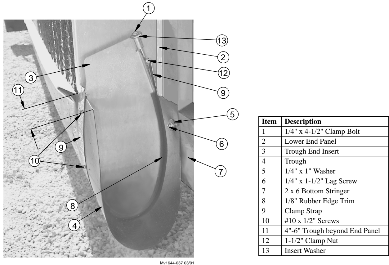
Figure 22. Trough End Insert Installation
