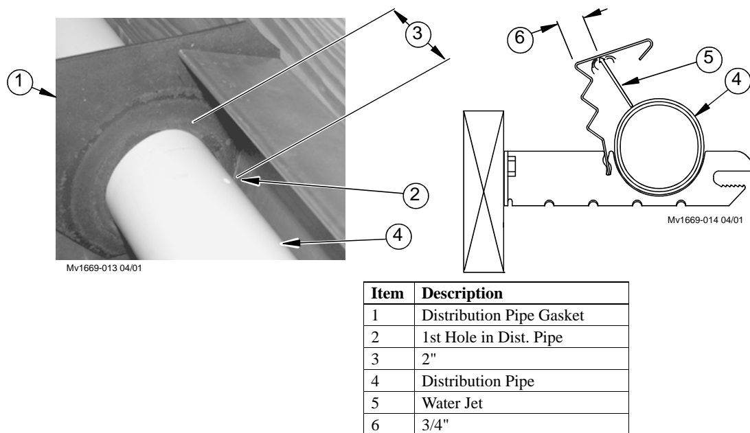
Figure 23. Orientating the Distribution Pipe
