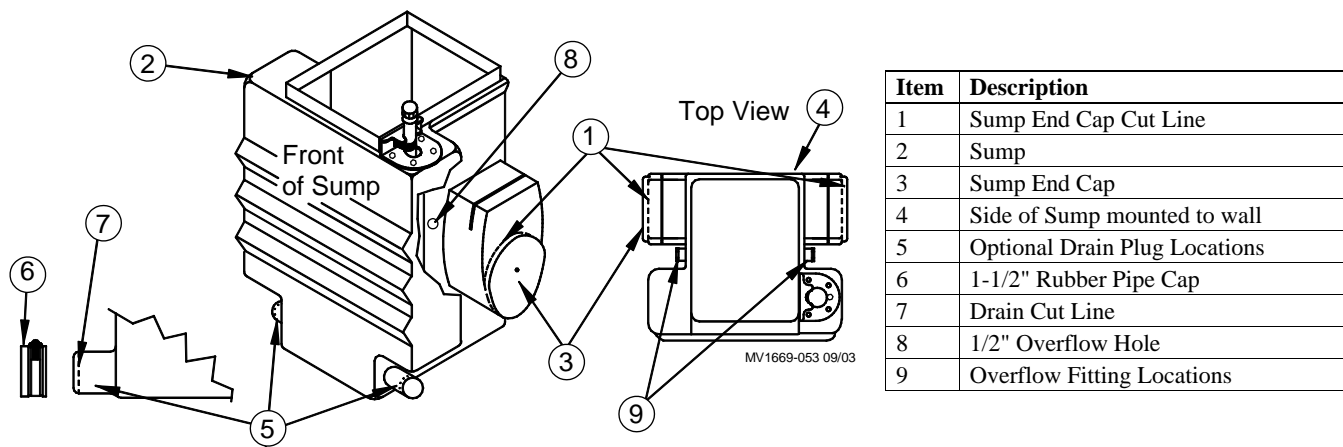
Figure 6. Cutting the Sump
