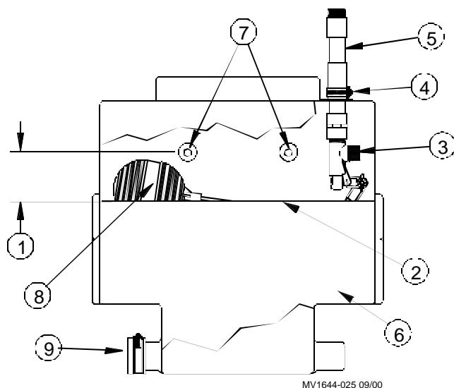
Figure 35. Adjusting Initial Water Level
