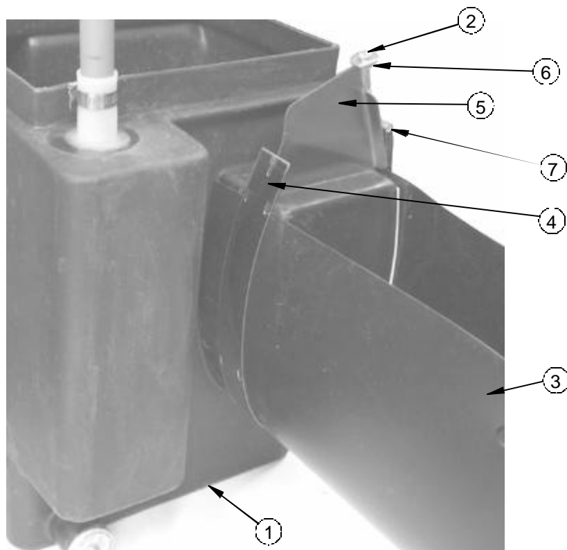
Figure 26. Sump End Insert Assembly
