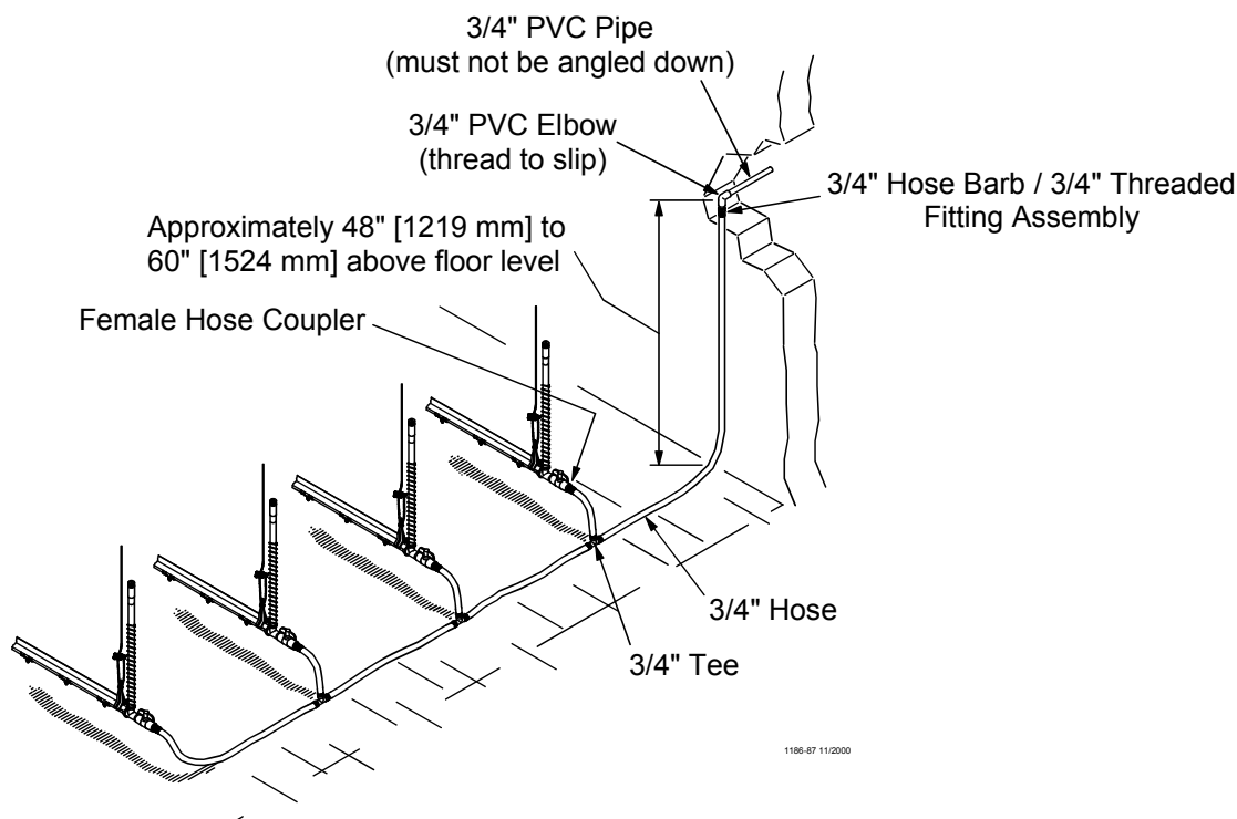
Figure 20. Flush System Component Layout Diagram
