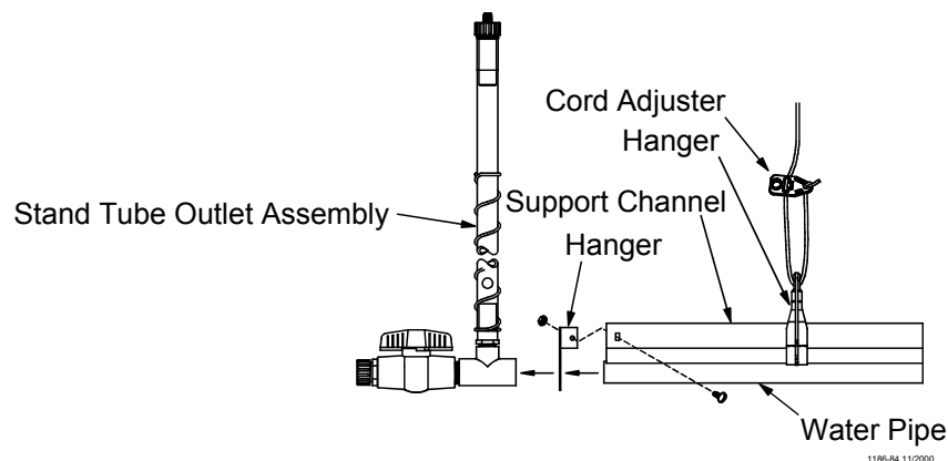
Figure 13. Outlet Assembly Installation
