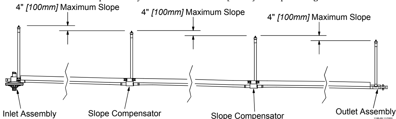
Figure 15. Slope Compensator Assembly Installation
