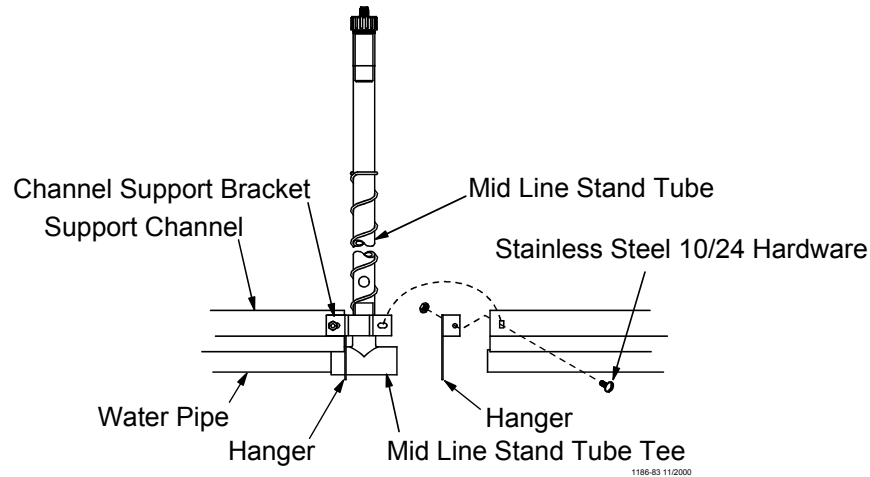
Figure 12. Mid Line Stand Tube Installation
