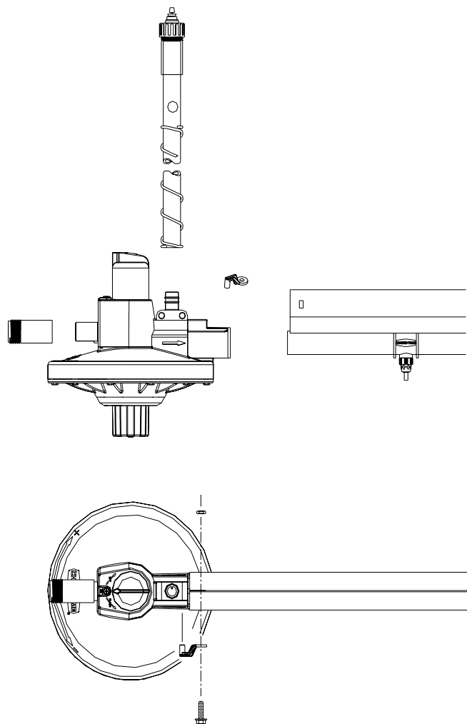
Figure 9. Inlet End Components
