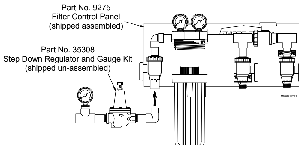
Figure 16. Control Panel Installation
