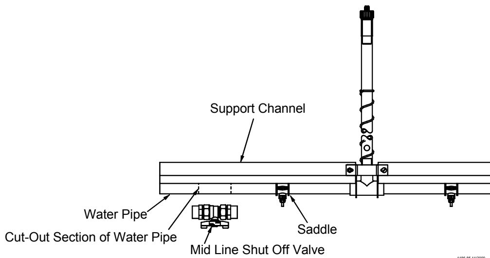
Figure 14. Mid Line Shut-Off Valve Installation
