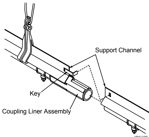
Figure 11. Securing the Water Line together
