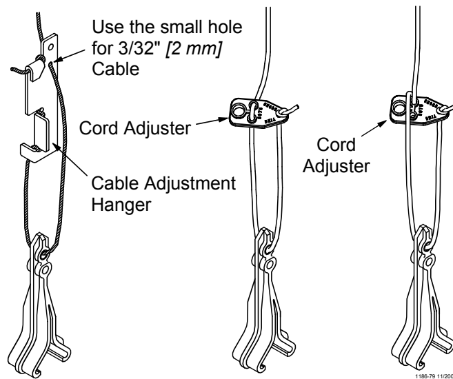
Figure 7A. Cable Drop Installation
