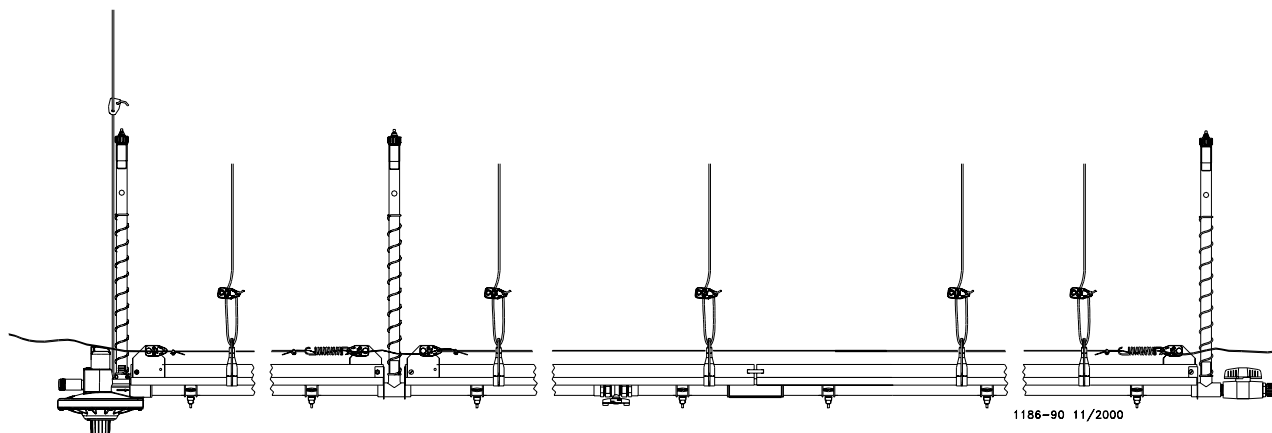
Figure 18. Anti-Roost System Overview
