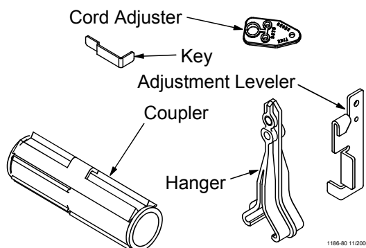
Figure 8. Nipple Waterer Components
