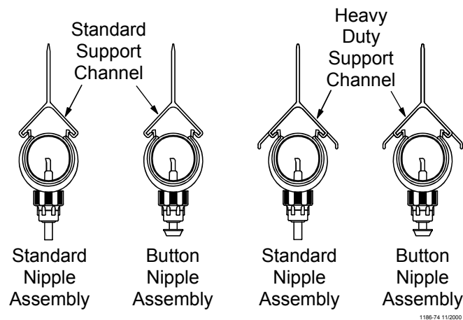
Figure 1. Various Drinker Styles (Side View)
