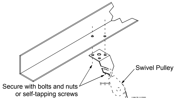
Figure 3. Ceiling Hook Installation (side view)
