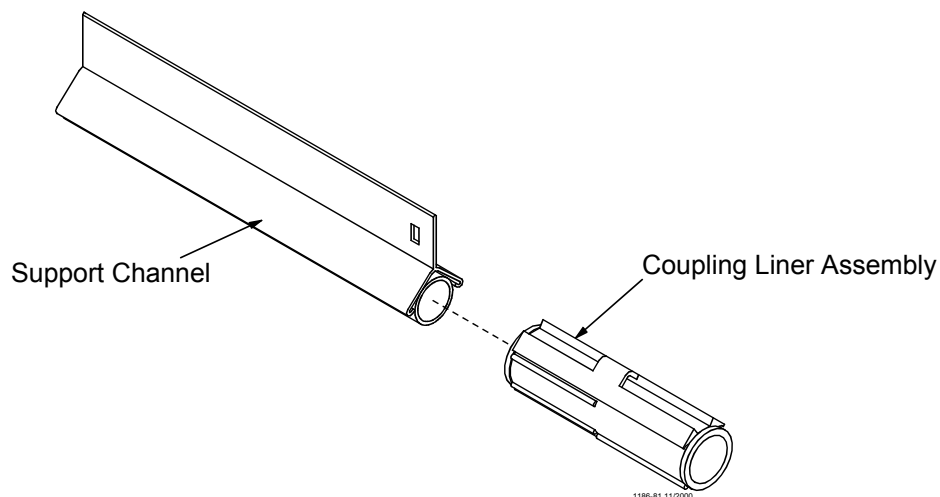
Figure 10. Coupling Liner Assembly Installation
