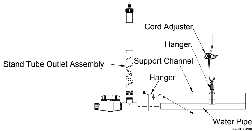
Figure 14. Outlet Assembly Installation
