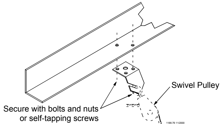
Figure 4. Ceiling Hook Installation
