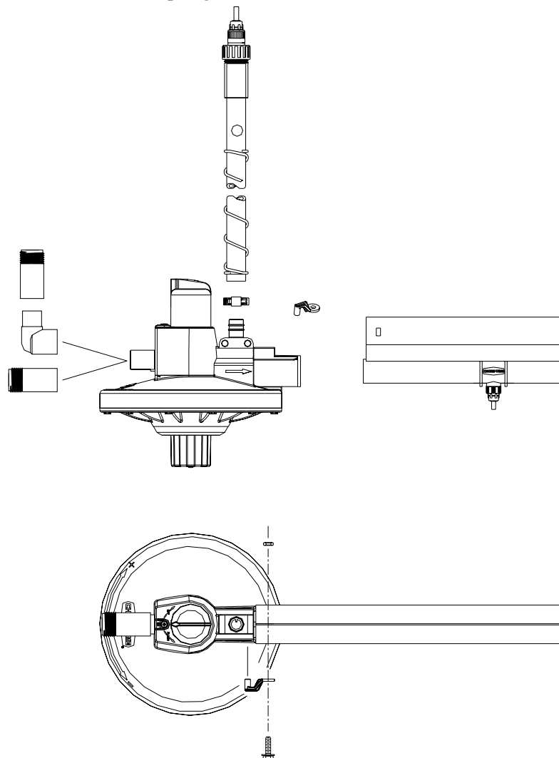
Figure 10. Inlet End Components
