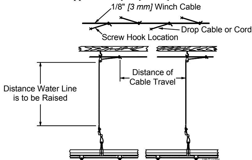
Figure 5. Offset the Screw/Ceiling Hooks
