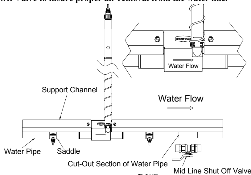
Figure 15. Mid-Line Shut-Off Valve Installation
