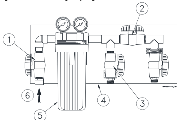
Figure 2. Cleaning or Changing Filter Cartridge
