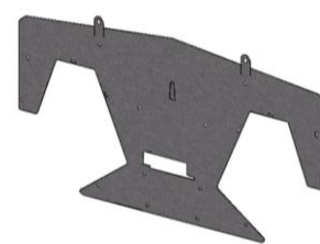
16550079 END PLATE OPPOSITE CONTROL END 1 each
