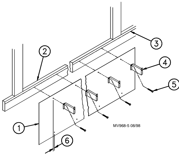
Figure 9. Installing the Trough
