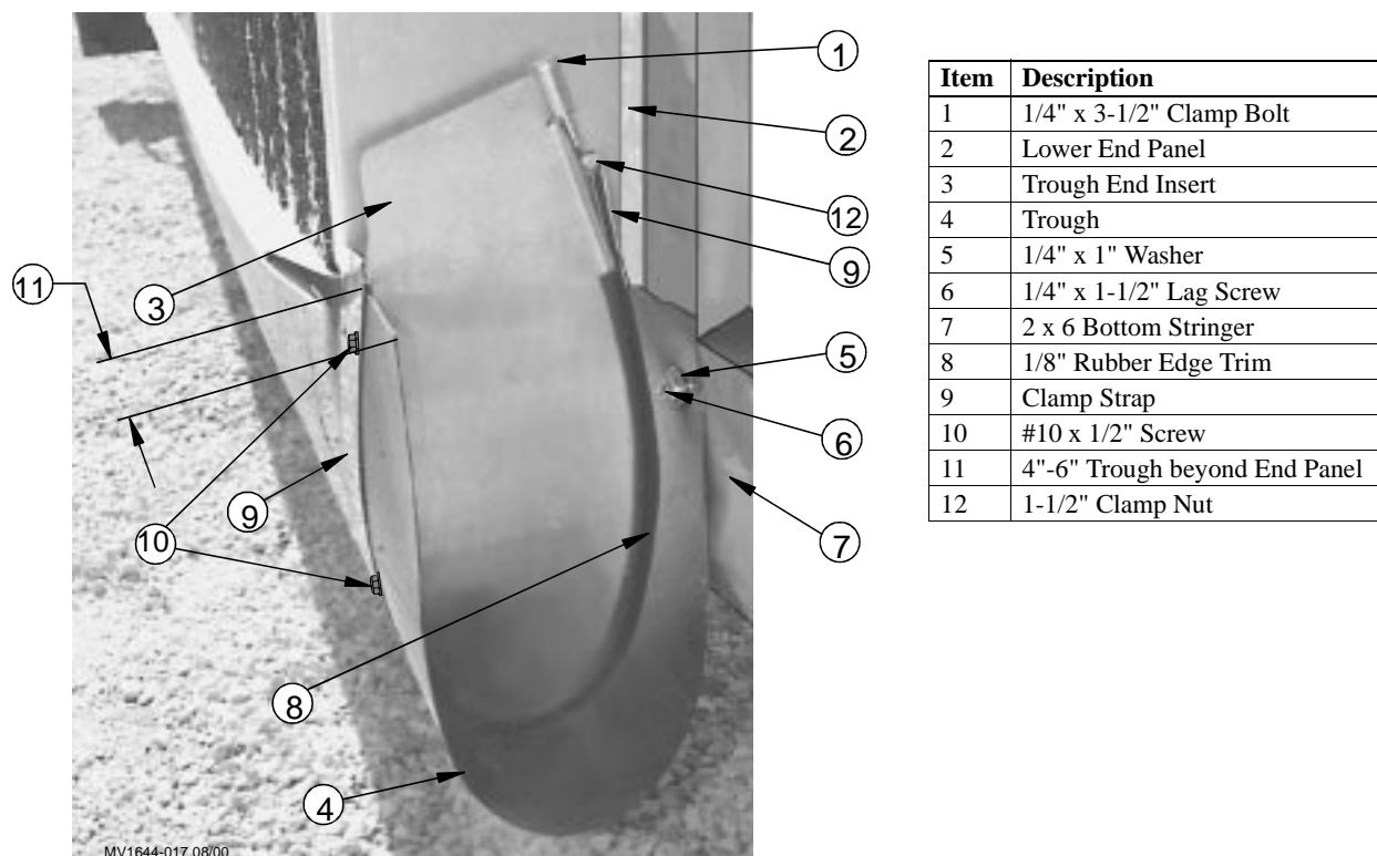
Figure 22. Trough End Insert Installation
