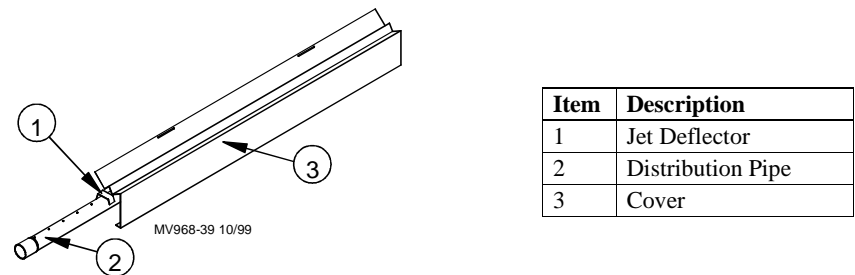
Figure 19. Jet Deflector
