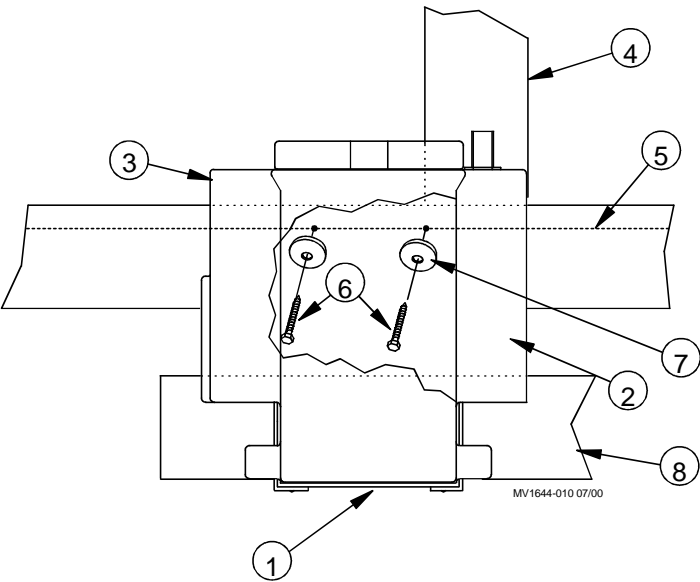
Figure 8. Attaching the Sump to the Bottom Stringer
