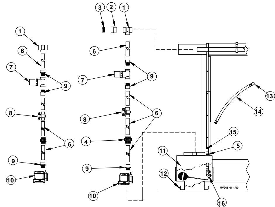
Sump in Center
