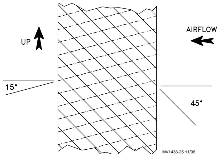
Figure 18. Pad Orientation (cut-away view of side of Pad)
