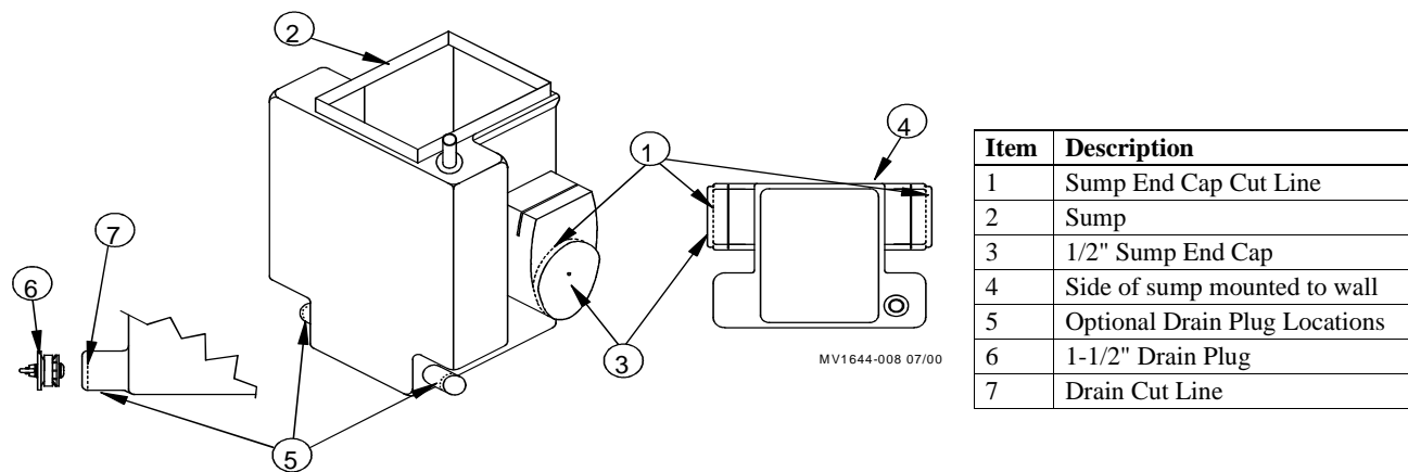
Figure 5. Cutting the Sump
