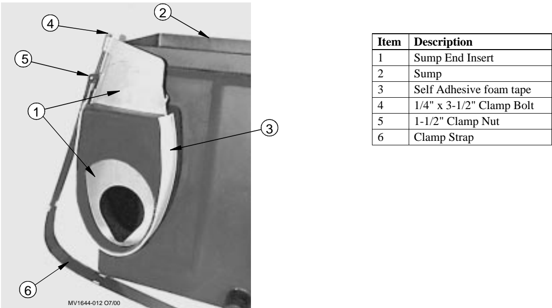
Figure 6. Sump End Clamp Assembly
