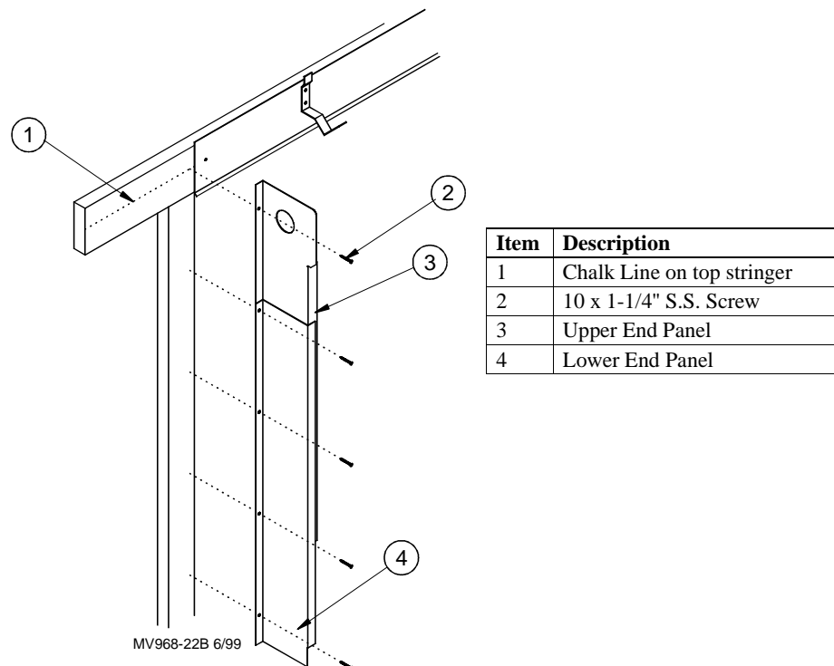
Figure 12. End Panel Installation
