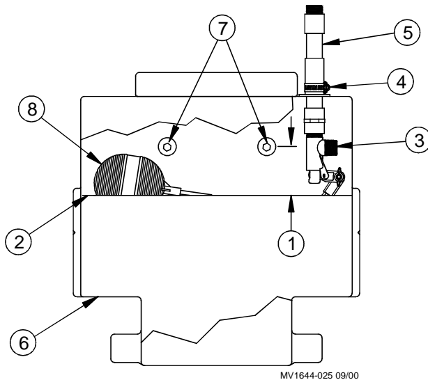
Figure 23. Adjusting Initial Water Level
