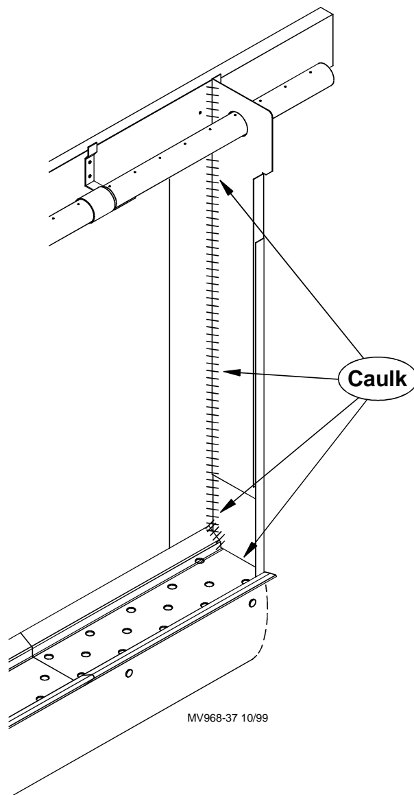
Figure 16. Caulking of rear joint of end panel
