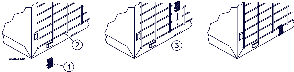
Figure 6. Screen Installation
