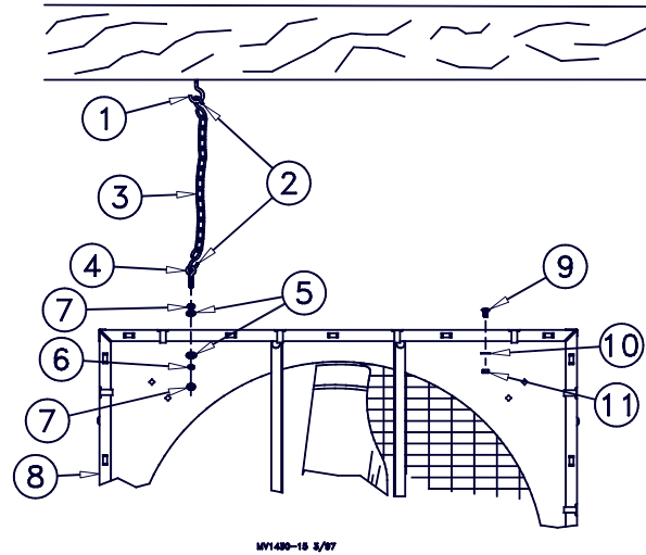
Figure 12. Suspending the Fan (front view)
