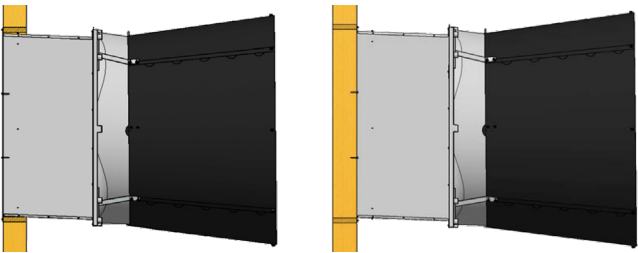
LEFT: Flush mount through the wall. RIGHT: Over the wall.
