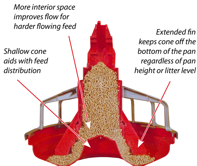
Chore-Time's MODEL C2® PLUS Extended Fin Feeder
