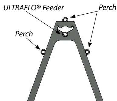
Ground-Supported Feeder Stand Option with Three Perches
